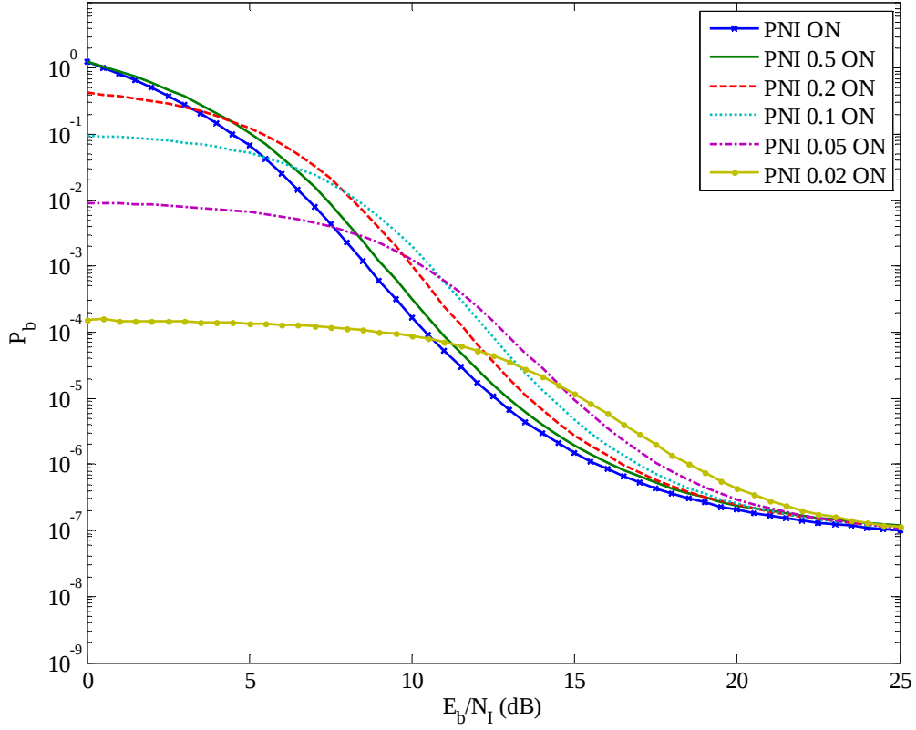
Figure 26. Performance of the alternative waveform in both AWGN and PNI with noncoherent demodulation and a diversity of two for \rho = 1 , \rho = 0.5 , \rho = 0.2 , \rho = 0.1 , \rho = 0.05 , and \rho = 0.02 when E_b / N_0 = 3.11 dB.
