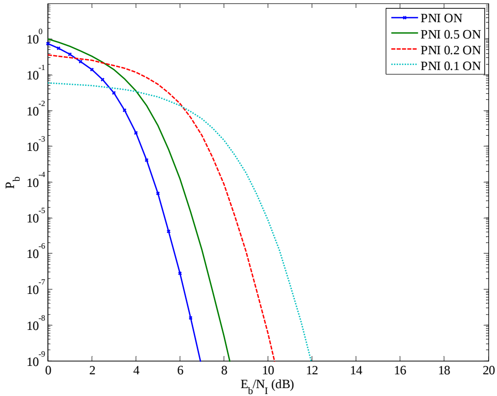
Figure 25. Performance of the alternative waveform in both AWGN and PNI with noncoherent demodulation with a diversity of two for \rho=1 , \rho=0.5 , \rho=0.2 , and \rho=0.1 when E_b / N_0 = 6 dB.
