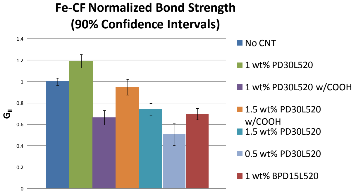
Figure 13. Normalized Bond Strengths of Steel-Carbon Fiber Bonds
