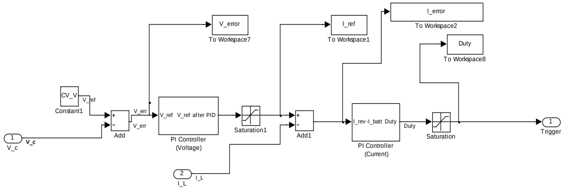
Figure 17. Controller Model.
