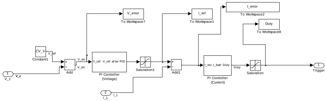
Figure 35. FPGA Controller Model.
