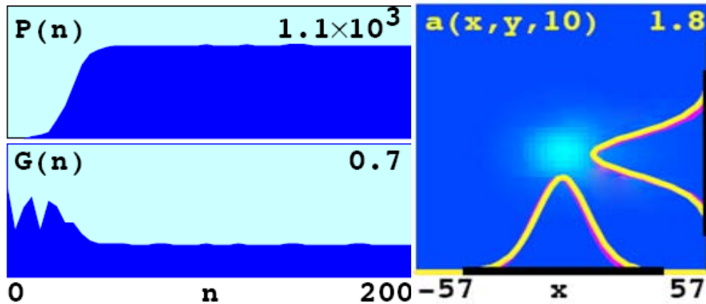
Figure 17. Top left is the power evolution and the bottom left is the gain evolution for the JLab FEL oscillator. Both are a function of number of passes, n=0 ->200 for this oscillator. On the right is optical field at the right mirror, which is aligned well with the fundamental Gaussian mode.
