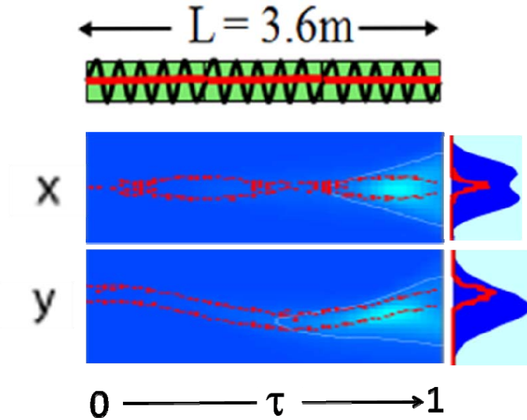
Figure 25. Generic FEL amplifier, showing the electron beam (red) and optical field (blue) as they progresses from \tau = 0 \rightarrow 1 . In red are sample electrons. The electron beam was shifted by 0.4 mm in the y direction. To the right of each picture are cross-sections vs. x and y of the electron beam and optical field.
