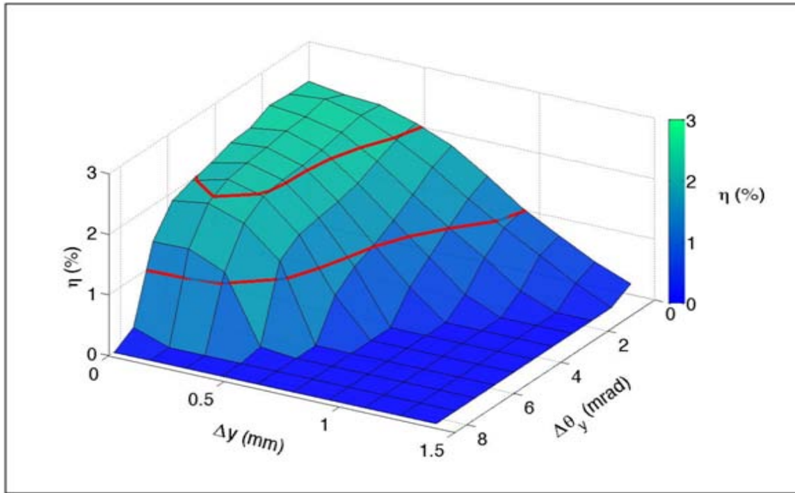
Figure 14. Extraction ( \eta ) versus both electron beam shift ( \Delta y ) and electron beam tilt ( \Delta\theta_y ). The red contour lines correspond to extractions of 1 and 2%.
