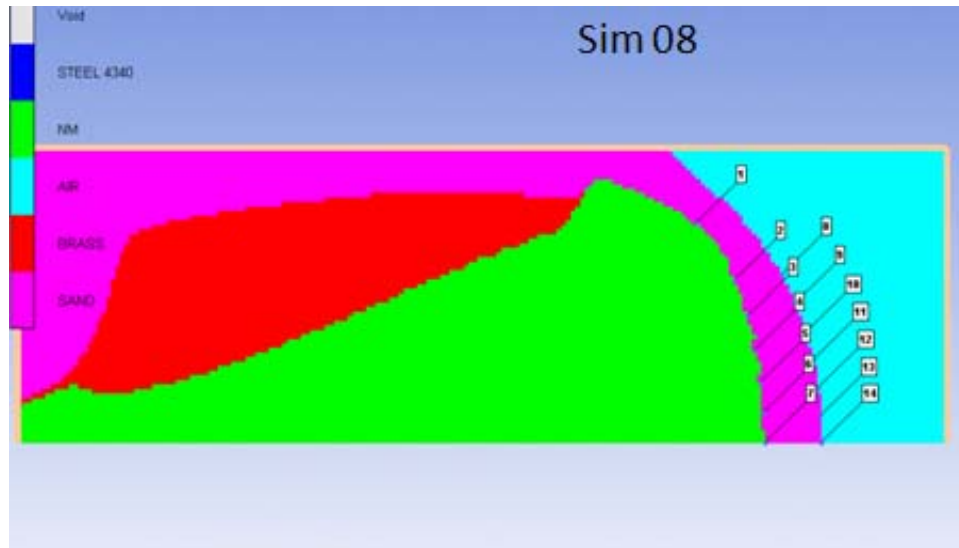
Figure 28. CC simulation with triangular shape of 20° angle.
