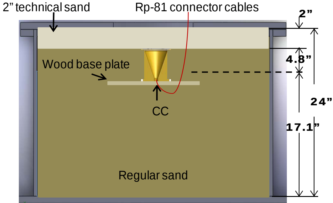
Figure 69. CC final configuration inside test chamber.
