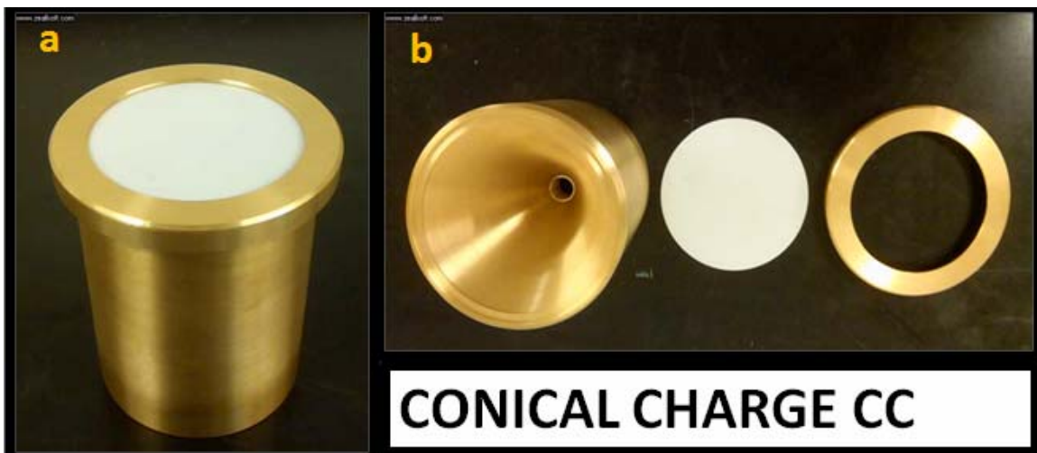
Figure 61. Actual pictures of CC, (a): partial assembly of LSTF, (b): top view showing CC main body with detonator seat at the bottom Teflon lid and top cap ring.
