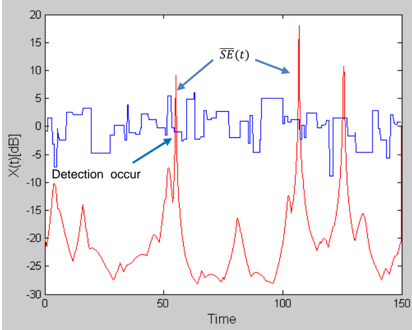
Figure 11. Example of (\lambda - \sigma) model simulation
