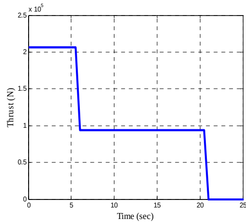
Figure 13. SM-6 Interceptor Thrust Profile
