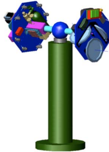
Figure 10. Virginia Tech Distributed Spacecraft Attitude Control System Simulator (DSACSS) (Whorl I, left; Whorl II, right) [From 27]
