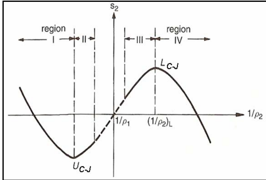
Figure 6. Entropy Distribution on the Hugoniot Curve (From [2]).
