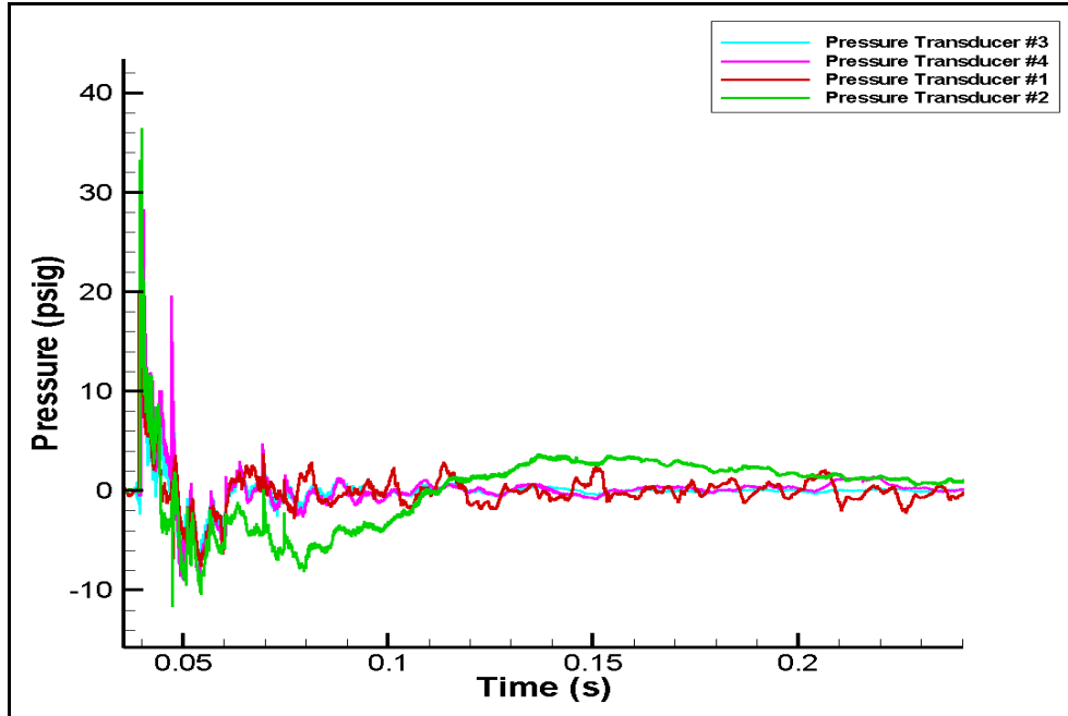
Figure 29. High-Speed Pressure Traces for Obstacle Free Configuration.
