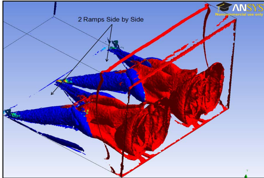
Figure 54. Ethylene Mass Fraction Vortices at Time 3.22E-4 sec.
