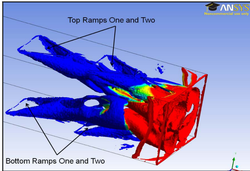
Figure 59. Ethylene Mass Fraction Vortexes at Time 6.31E-4 sec.
