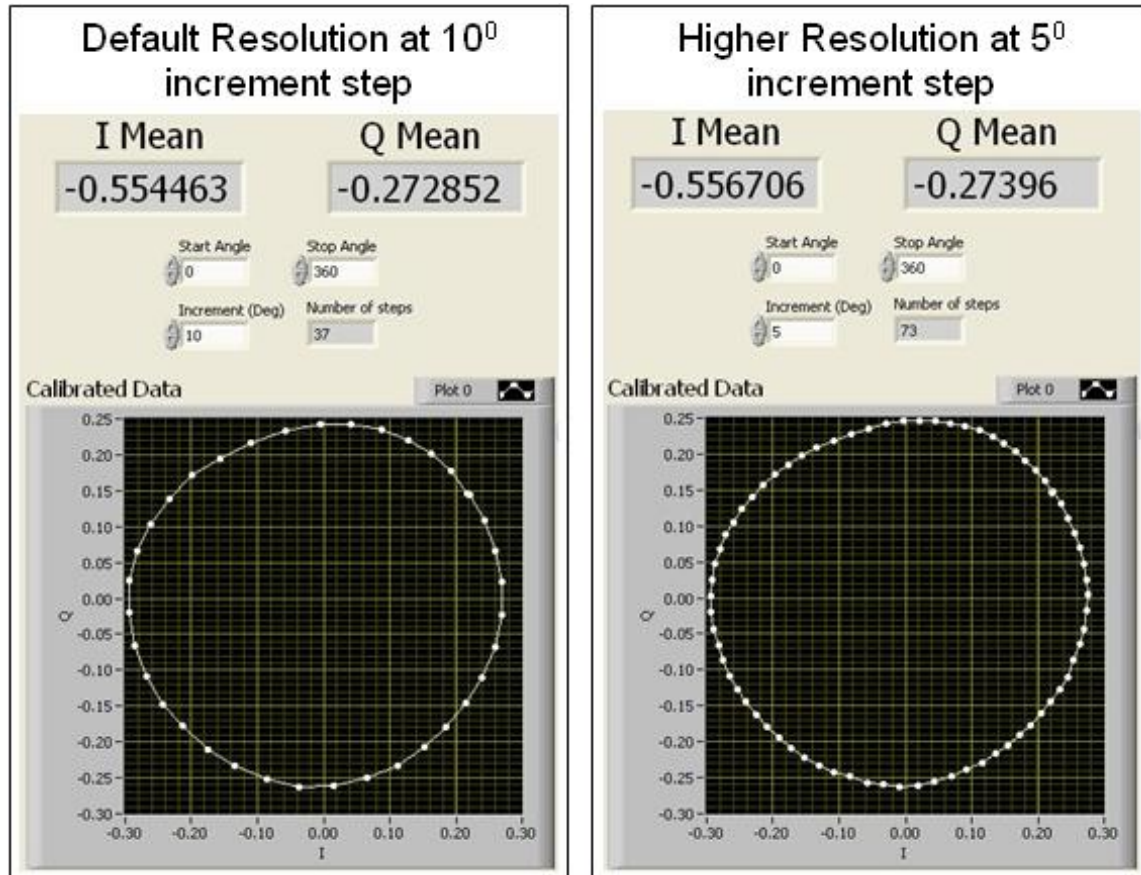
Figure 70. I and Q Circle at 10^\circ and 5^\circ Increment Step.
