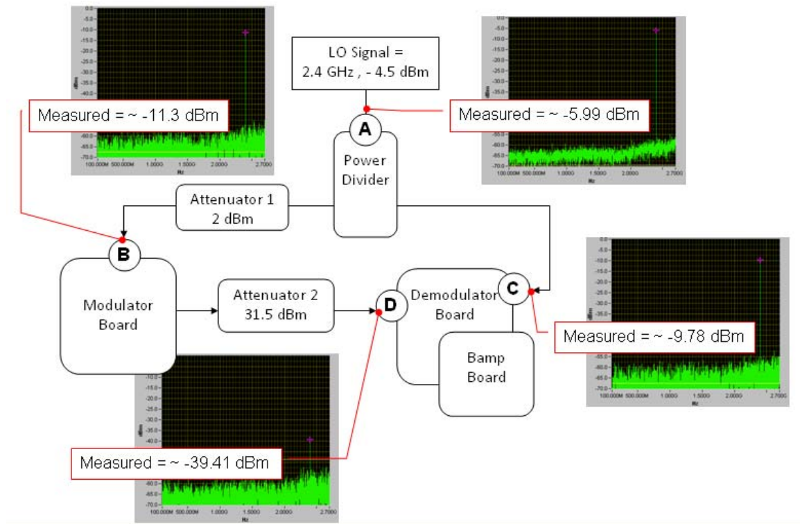
Figure 40. Attenuation Measurement.
