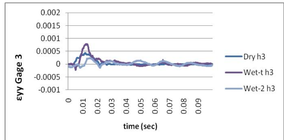
Figure 50. Representative \epsilon_{yy} gage 3 response at 3.9 m/sec velocity
