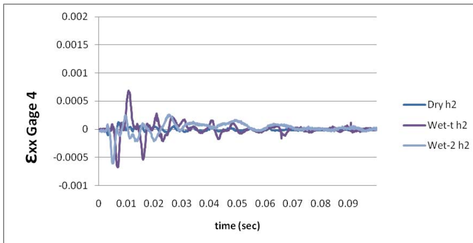
Figure 40. Representative \epsilon_{xx} gage 4 response at 3.9 m/sec velocity
