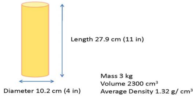
Figure 4. Cylindrical modem dimensions
