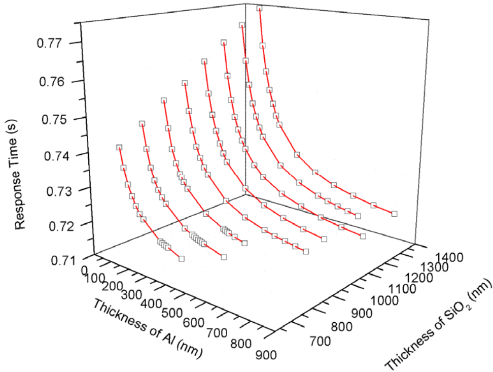
Figure 14. 3D graph of the response time by varying the Al and SiO 2 thicknesses
