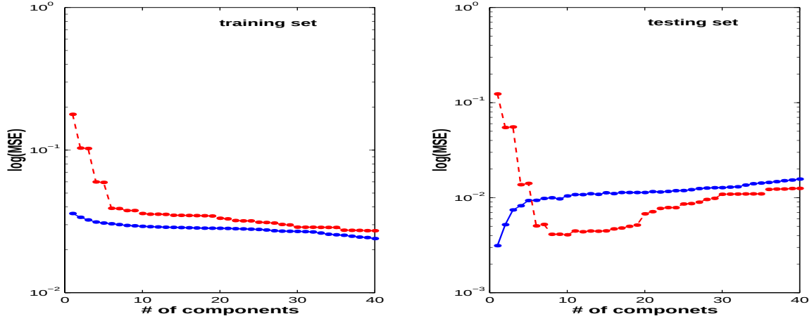
Figure 2: Sinc function approximation. Dependence of the training and testing error of kernel PLS (solid line) and kernel PCR (dashed line) on the number of extracted components. Gaussian noise with standard deviation equal to 0.2 was added to the training data set outputs. Error is evaluated in terms of mean squared error (MSE).
