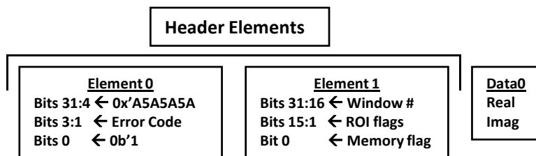
Figure 37. Header Format with Error Code.
