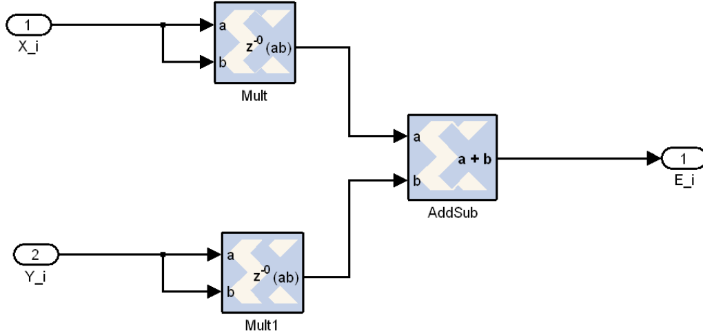
Figure 13. Circuit to Calculate Energy(k) [From 3].
