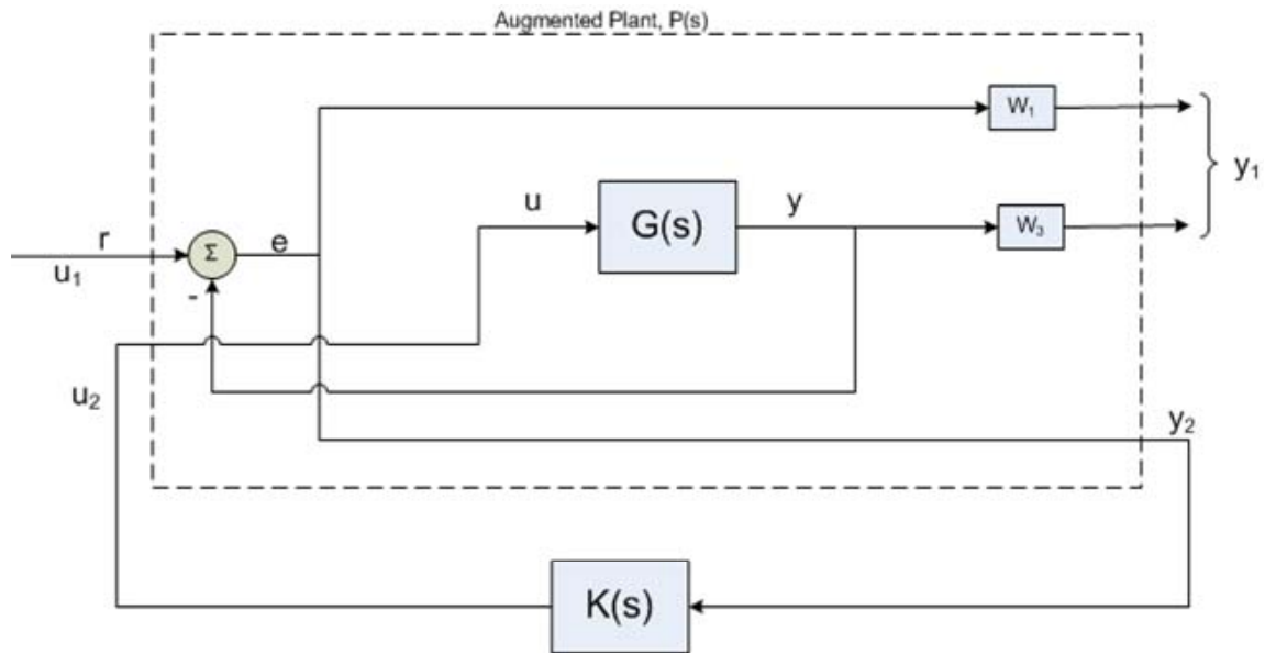
Figure 41. H_\infty Controller and Augmented Plant
