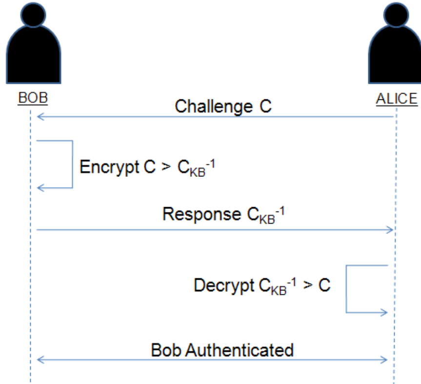
Figure 4. Authentication Process
