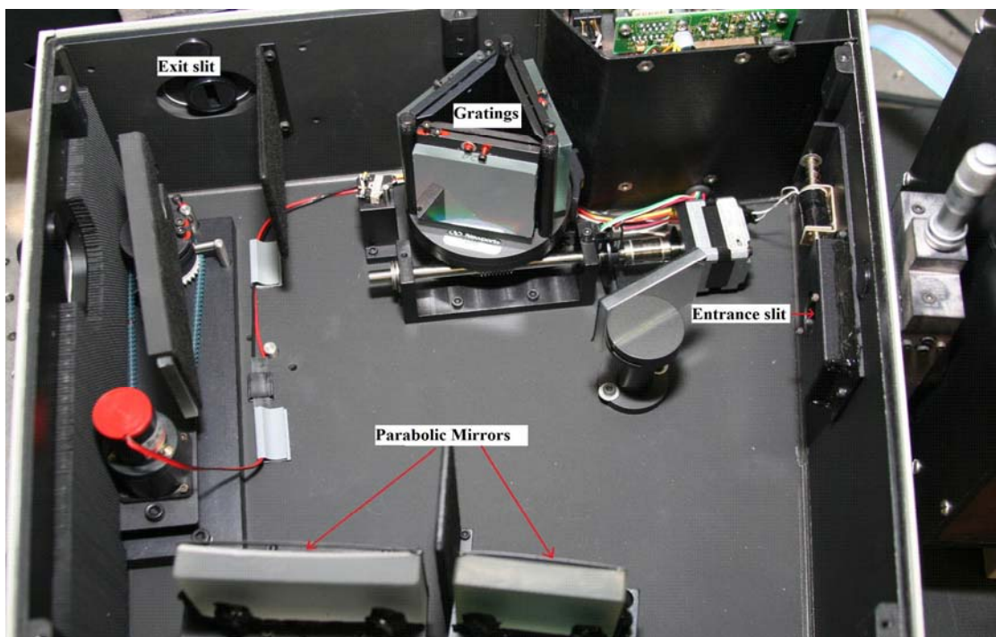
Figure 20. Monochromator (Oriol Cornerstone 260 ¼).
