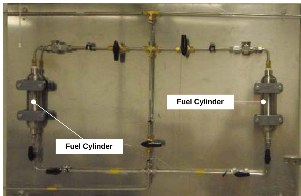
Figure 23. Fuel Cylinders
