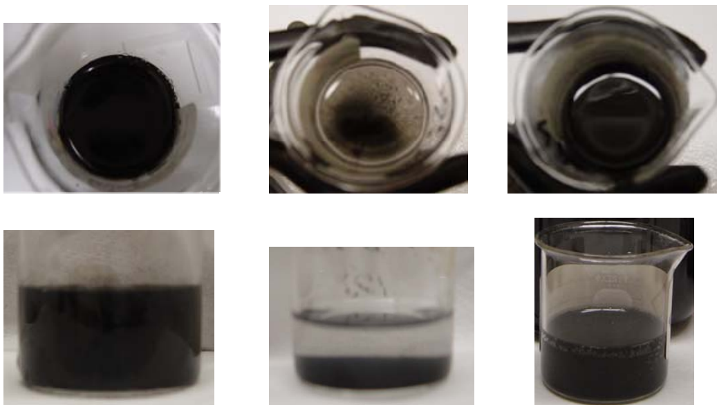
Figure 16. (Left) Initial Appearance of LnW-402. (Middle) Appearance of LnW-402 after 12th Cycle. (Right) Appearance of LnW-402 after Re-sonication
