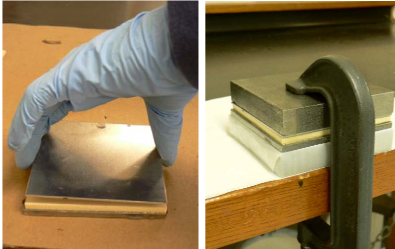
Figure 31. Photos Illustrating the Placement Process as well as the Application of Uniform Pressure over the Sample Using Top and Bottom 20mm Mild Steel Plates
