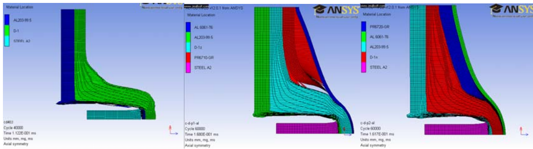
Figure 60. Comparative Autodyn® Simulation of the Three Composite Plates, C-D1, C-D1-P1-A1, and C-D1-P2-A1, Subjected to Same Projectile Impact at 483 m/s
