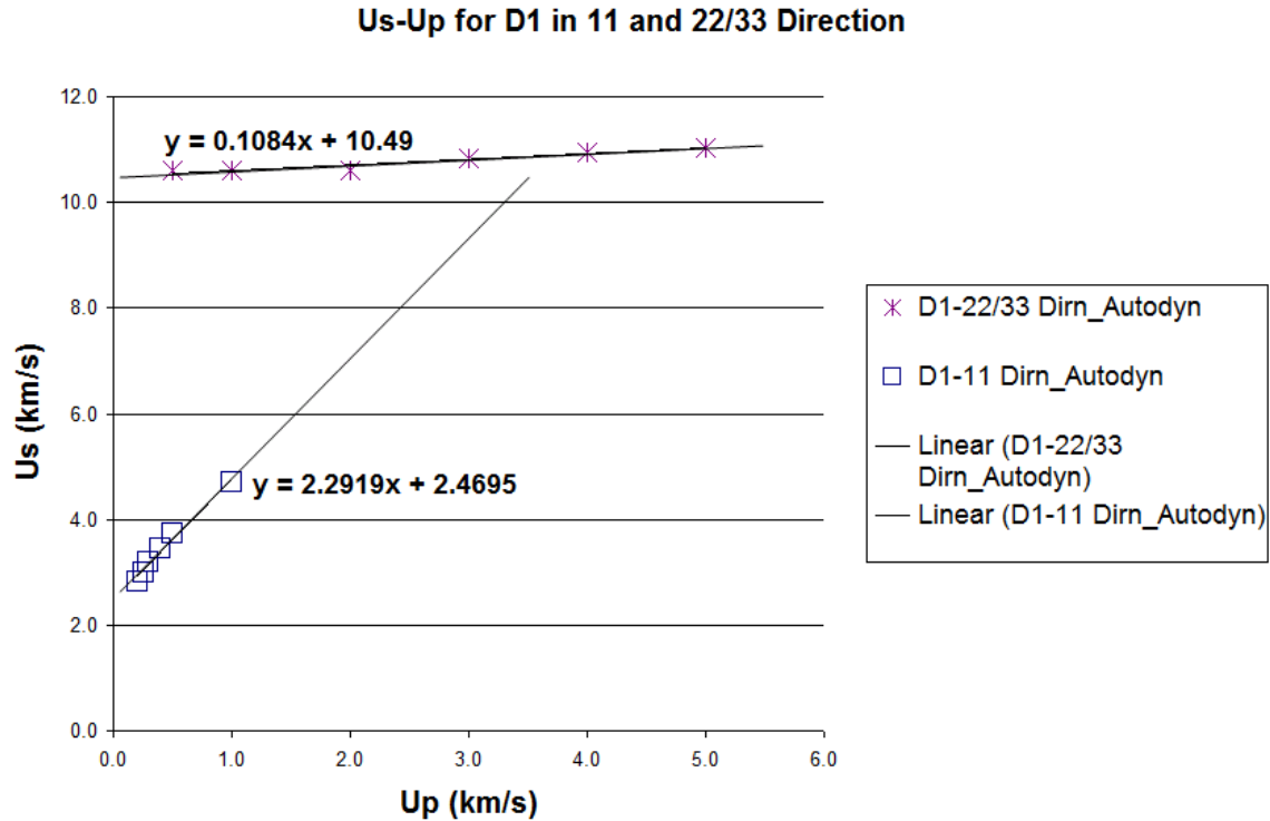
Figure 24. Us-Up relationship of the D1 Material in the 11- and 22/33- directions
