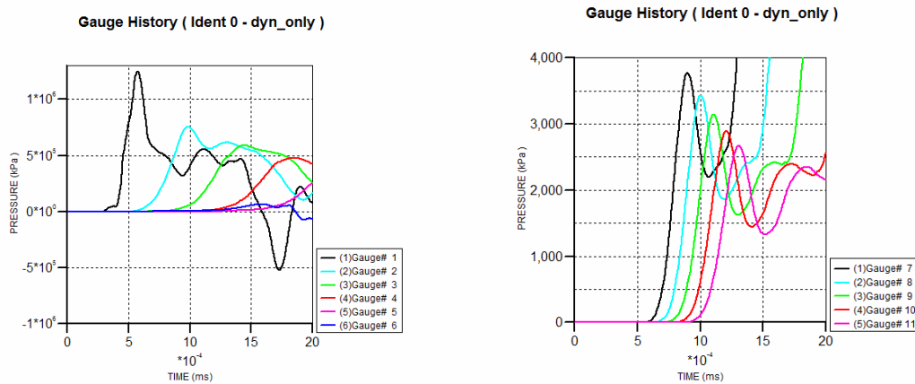
Figure 48. (Left) Shockspeed of 3.0 km/s was seen to propagate in the 11 direction. (Right) In the 22/33 directions, the shockspeed was 9.9 km/s.
