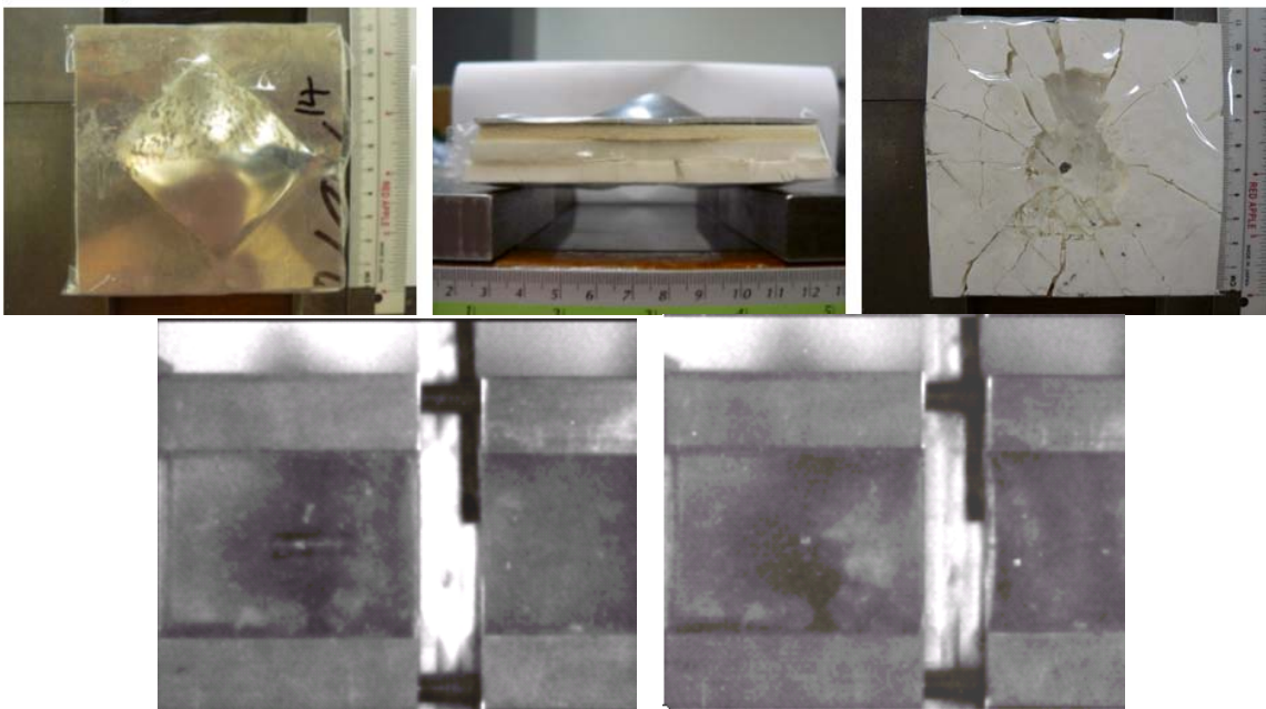
Figure 44. Sample of C-D-P1-Al Showing Complete Fracture of the Ceramic First Layer, and no Penetration of the Projectile.
