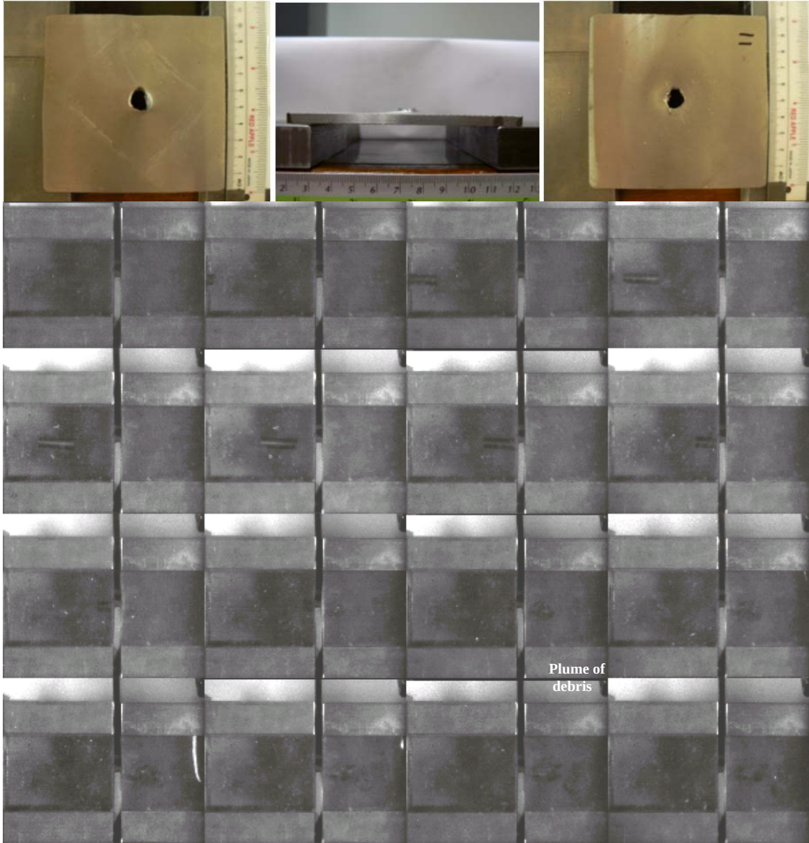
Figure 41. Target Samples and High Speed Camera Frame Photographs and the Associated Damage of the AISI 4140 Steel Plate Impacted with 1" A2 Projectile at 484m/s.
