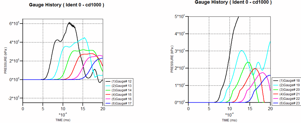
Figure 27. (Left) Ceramic Shock Profile in the 22/33-direction. (Right) D1 Shock Profile in the 22/33-direction.
