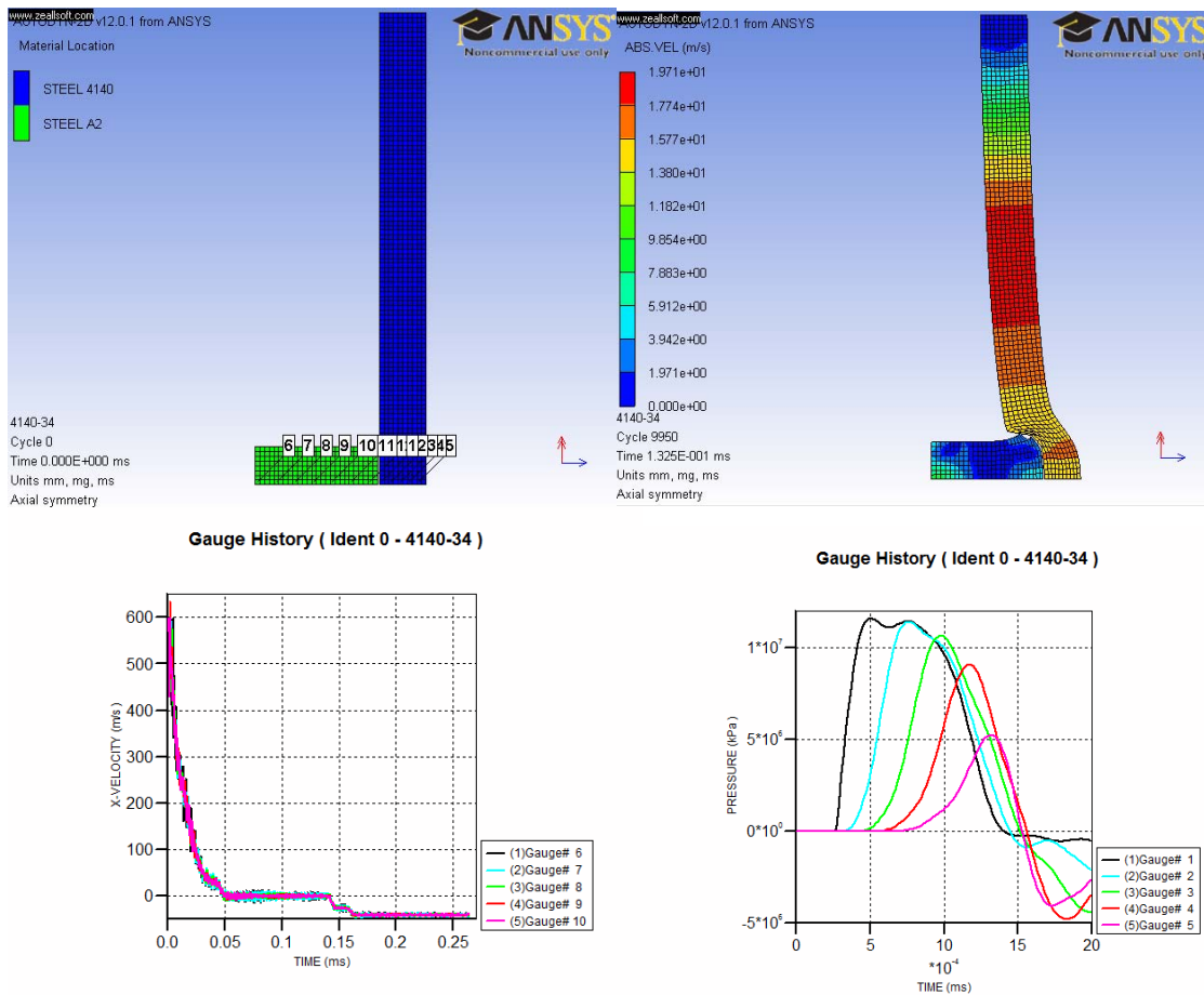
Figure 49. Results of Autodyn® Simulations of a ½” A2 Cylinder Projectile Impacting AISI 4140 Steel at 596m/s. (Top Left)Problem Setup of a ½”A2 Steel Cylinder Impacting at 595 m/s onto a AISI 4140 Steel Plate. (Top Right)Projectile is stopped by the Steel Plate. (Bottom Left)Velocity Profile of the Steel Projectile. (Bottom Right)Pressure-Time Profile in the Target Steel Plate.
