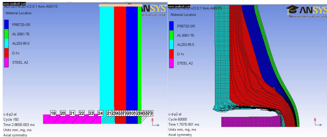
Figure 58. Problem Set up of C-D1-P2-AL Composite Plate. Impact Velocity of 463m/s. Final Deformation Shape is Shown on the Right. .
