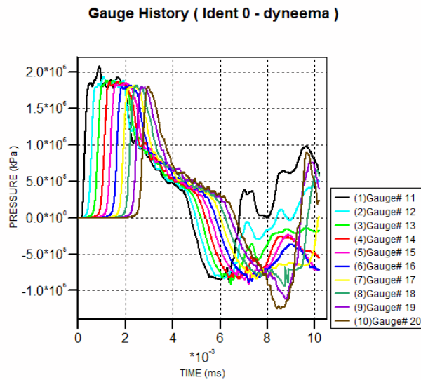
Figure 17. Overall Shock Wave Profile in the 11-direction
