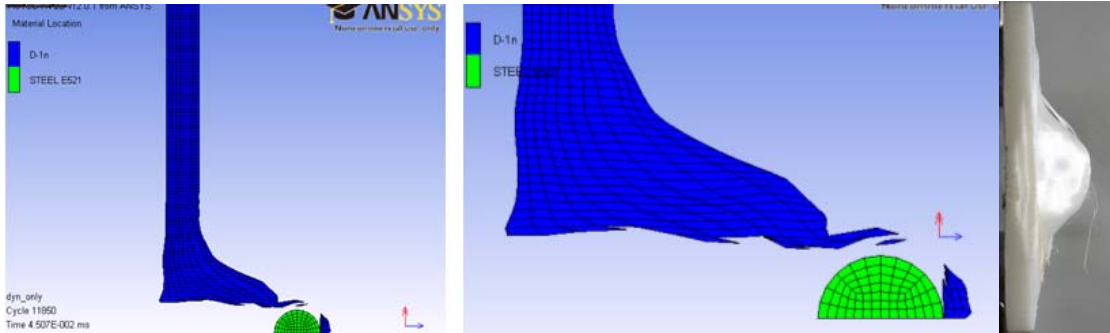
Figure 47. End State of Autodyn® Simulations Showing Complete Penetration with 275 m/s Residual Velocity. The Actual Damage Sample is on the Right for Comparison Purposes.
