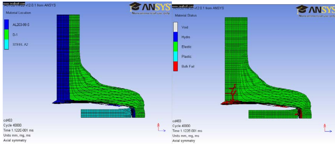
Figure 53. Results of Autodyn® Simulations of Composite Plate (C-D1). (Left) Final Deformation Shape of the Composite Plate. (Right) Bulk Failure and Brittle Fracture of the Ceramic Plate can be observed.
