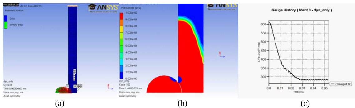
Figure 46. D1 Problem Setup. Impact Velocity was the Same as That of the Experiment – 610m/s. (a) Problem Setup of a 9/32” E52100 Steel Ball impacting a D1 Target. (b) Shock Wave Propagation at 1.5µs after Impact. (c) Simulation Residual Velocity was 275 m/s.
