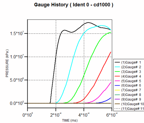
Figure 26. Ceramic Material Results. 17.3 GPa Peak Pressure is Observed, with a 3.45km/s Shock Velocity in the 11-direction
