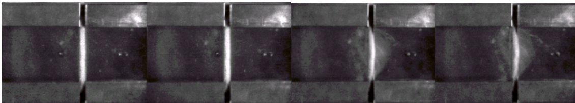
Figure 37. High-speed photos showing Dyneema before and after penetration by steel sphere.
