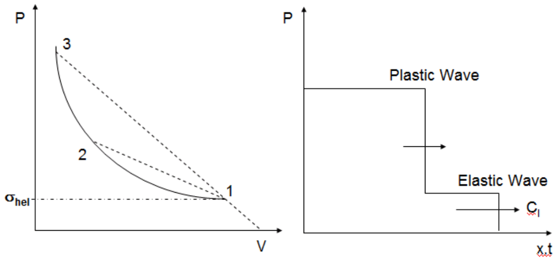
Figure 22. Explanation of the Difference between the Elastic and Plastic Wave Speed. (From [21])
