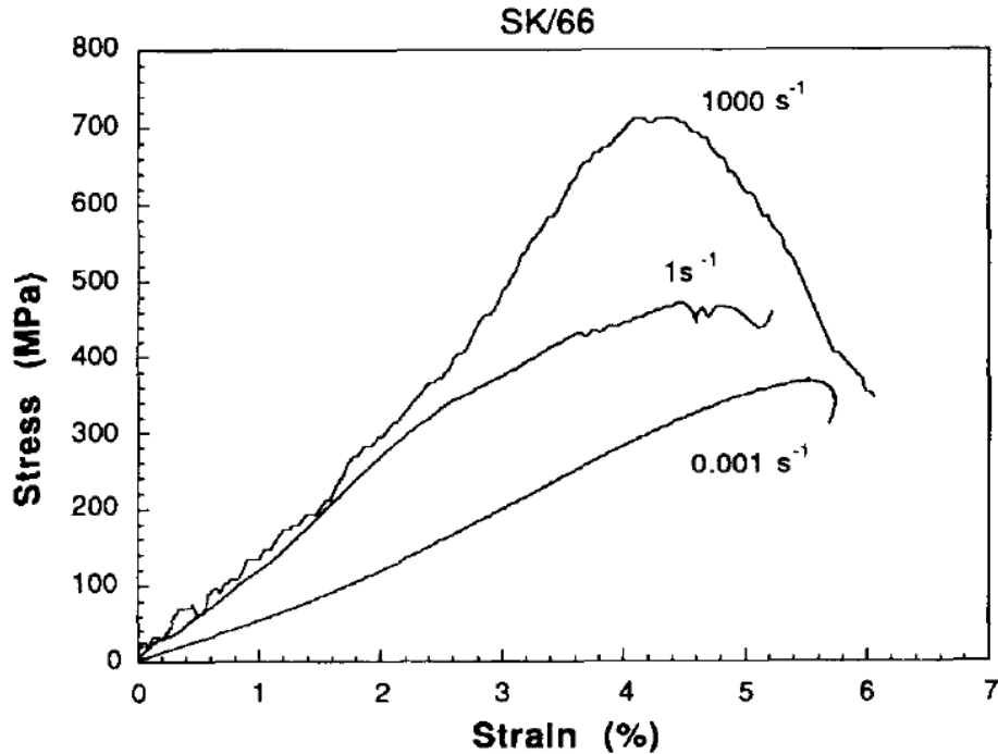
Figure 8. Stress-strain Behavior of Dyneema Fibers at up to Strain Rates of 1000s-1 (From [14])
