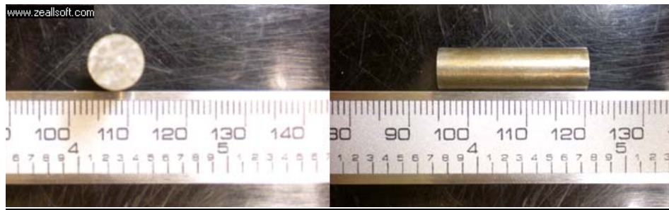
Figure 30. A2 Tool Steel Cylinder Projectile that was Used in the Experiment. (Rockwell Hardness C 55-56. Yield Strength of 1.8 GPa)
