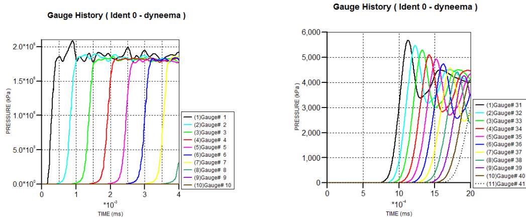
Figure 18. (Left) Rise Times of the Shock Wave Propagating in the 11-direction. (Right) Rise Times of the Shock Wave Propagating in the 22/33-directions
