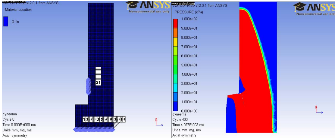
Figure 16. Set up of a D1-D1 Symmetric Impact of a Bullet on a Larger Target Plate. (Left) Gages are setup in the 11- and 22-directions. (Right) Lateral wave speed is seen to be faster than the through thickness wave speed as exhibited by the shock front.
