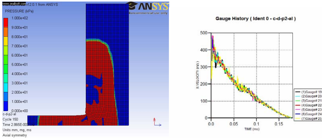
Figure 59. Shock Wave Propagation in the 11 and 22 directions. Time Taken to Arrest the Projectile was 0.177ms
