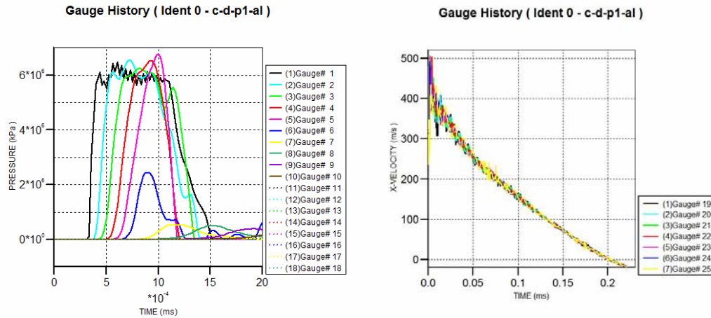
Figure 57. (Left) Peak Pressure Profiles Obtained During the Initial Stages of Impact. (Right) Time Taken for Projectile to Reach Zero Velocity was 0.2 ms.
