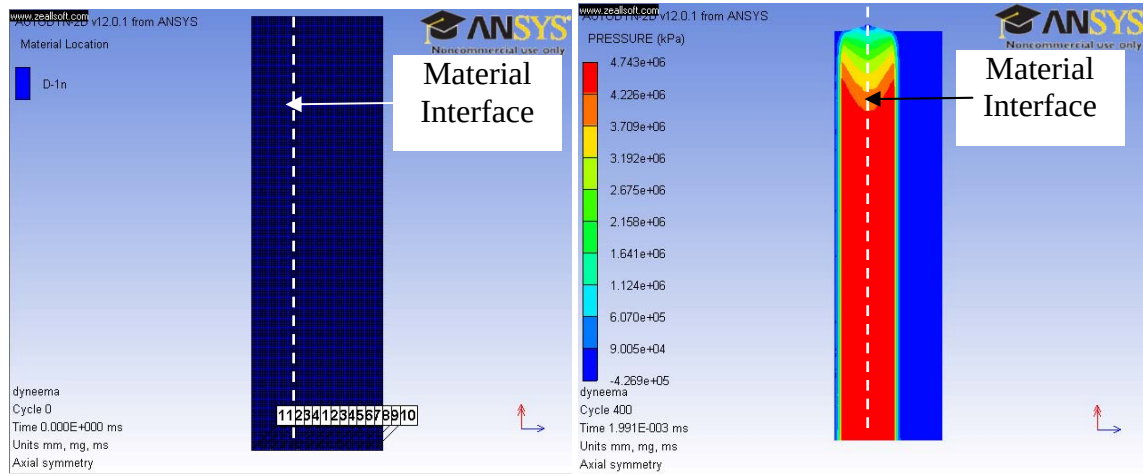
Figure 14. Symmetric Plate Impact of D1 Material at 1 km/s. Plates were 200mm Cylindrical Plates of 5 mm and 10 mm Thickness Respectively. (Left) Problem Setup. (Right) Planar Wave Propagation at 2 \mu s after Impact.
