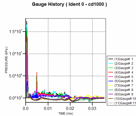
Figure 25. Autodyn® Simulation of an A2 Steel Cylinder Bullet Impacting at 1000m/s onto a Ceramic-D1 Composite Plate. (Left) Problem setup. (Right) Overall Pressure-Time profile.
