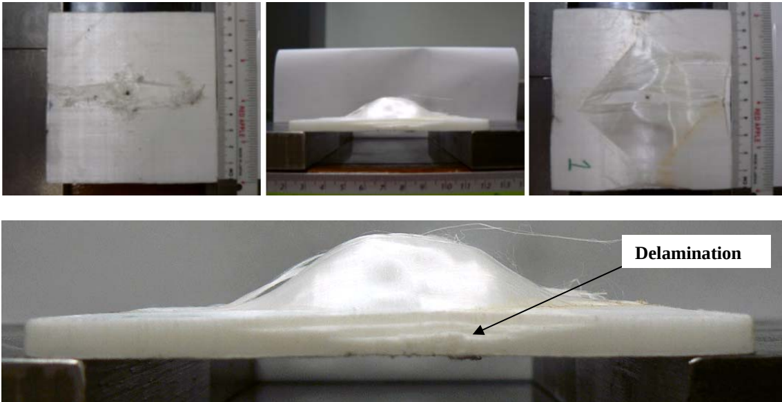
Figure 36. Samples of Dyneema HB25 Showing Full Penetration by an E52100 9/32" Steel Ball.
