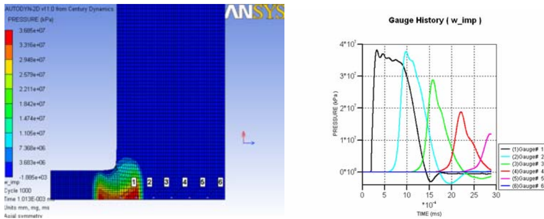
Figure 12. Shock Pressure Profile of the W-Ta Plate Impact (Impact velocity was 1000m/s)
