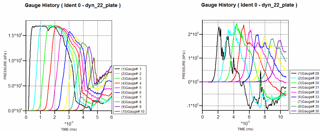
Figure 20. (Left) Shock Profile in the 22-direction. (Right) Shock Profile in the 11-direction.
