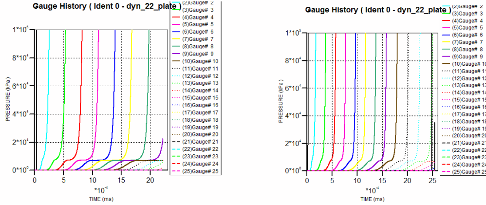
Figure 23. (Left) Plastic Wave at 5km/s Impact Velocity. (Right) Plastic Wave at 10km/s Impact Velocity.
