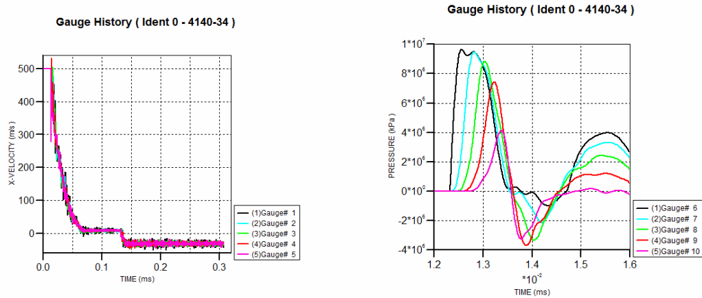
Figure 50. Results of Autodyn® Simulations of a \frac{3}{4} " A2 Cylinder Projectile Impacting AISI 4140 Steel at 500m/s. Peak Interfacial Pressure was 9.52 GPa. (Top Left) Problem Setup of a \frac{3}{4} " A2 Steel Cylinder Impacting at 500 m/s onto a AISI 4140 Steel Plate. (Top Right) Projectile is stopped by the Steel Plate. (Bottom Left) Velocity Profile of the Steel Projectile. (Bottom Right) Pressure-Time Profile in the Target Steel Plate.
