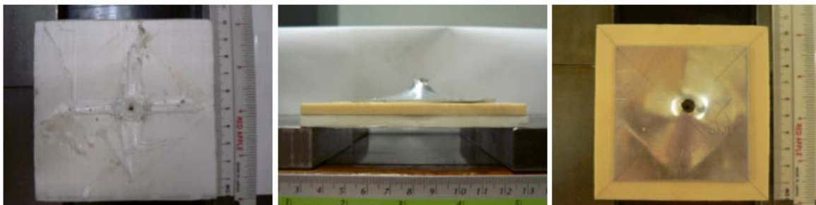
Figure 38. Addition of a Shock Porous Foam in the Rear did not Appear to Help in Resisting Penetration as Can be Seen from the Similar Exit Velocity of the Projectile.
