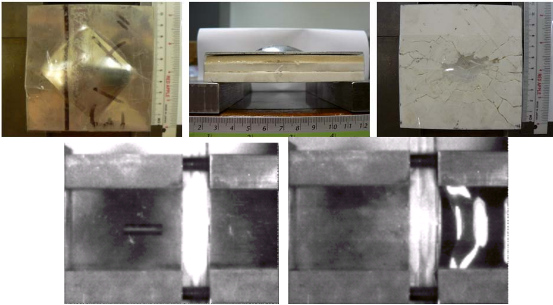
Figure 43. Sample of C-D-P2-Al Showing Complete Fracture of the Ceramic First Layer, and no Penetration of the Projectile.
