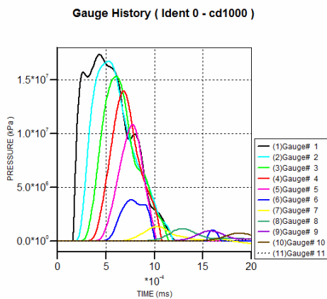
Figure 26. Ceramic Material Results. 17.3 GPa Peak Pressure is Observed, with a 3.45km/s Shock Velocity in the 11-direction
