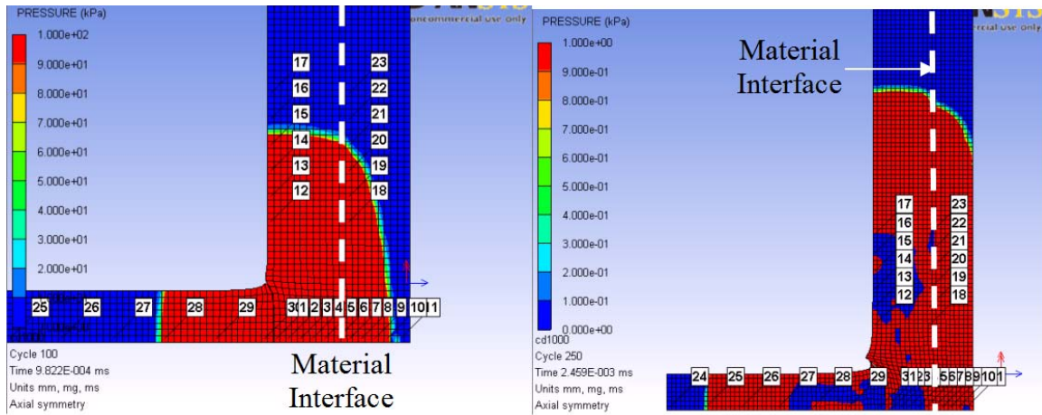
Figure 28. Shock Wave Propagation is Slowed Down in the 11-direction Due to the Presence of the D1 Material
