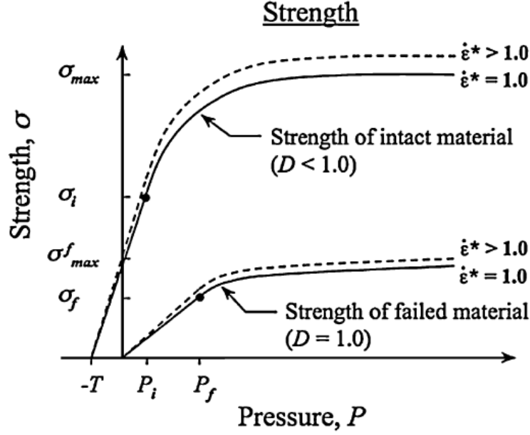
Figure 7. Strength Model for Ceramic Materials. (From [7])
