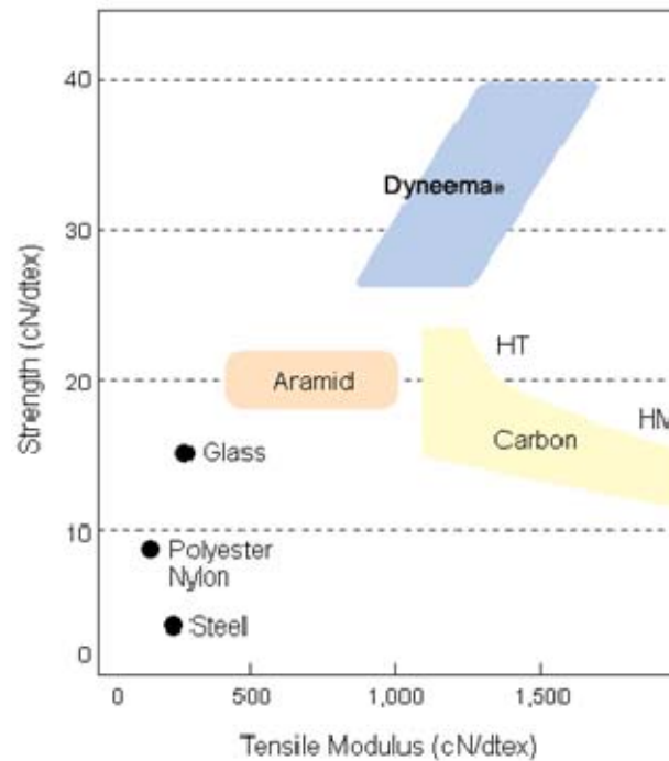
Figure 2. Relative Strength/ Tensile Modulus of Advanced Fiber Composites (From [2]) Note that units are in centi-Newtons/decitex, which is the load per unit line density. 1 decitex is the weight in grams of 10,000m of a single strand of fiber.
