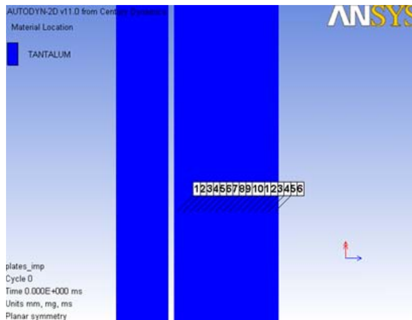
Figure 10. Autodyn® Problem Set Up Of Tantalum Flyer Plate Impact
