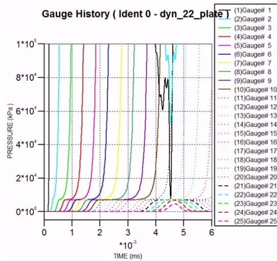
Figure 21. Elastic Wave Moving Ahead of Plastic Wave in the 22-direction.
