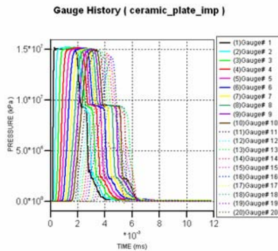
Figure 13. Pressure Profile of Ceramic-Ceramic Flyer Plate Impact at 1000m/s
