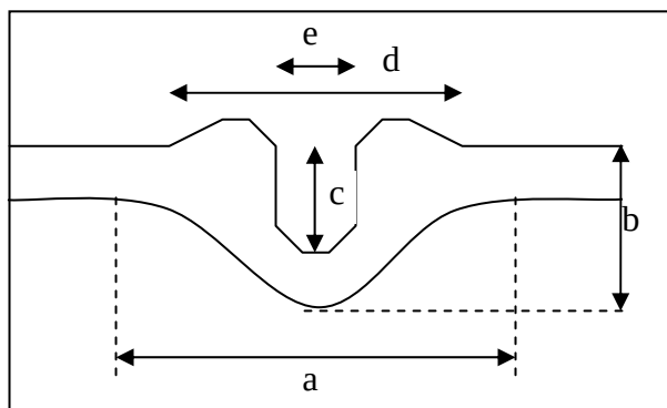
Figure 45. Dimensions that were measured using a 1/1000th accuracy Vernier Calipers
