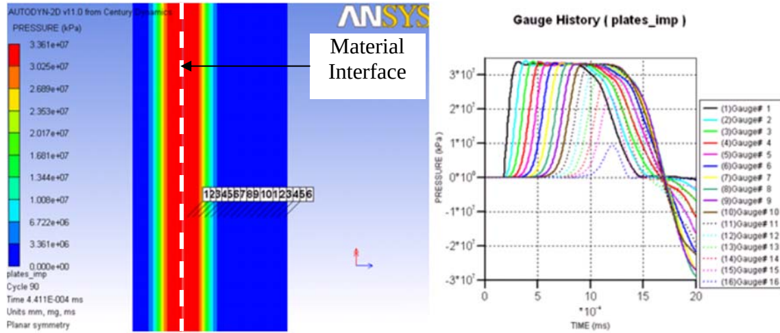
Figure 11. Shock Pressure Profile of the Ta-Ta Plate Impact (Impact velocity was 1000m/s)
