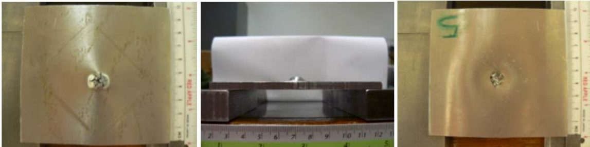
Figure 39. Target Samples and the Associated Damage of the AISI 4140 Steel Plate Impacted with 1/2" A2 Projectile at 596m/s. No Penetration was Observed.
