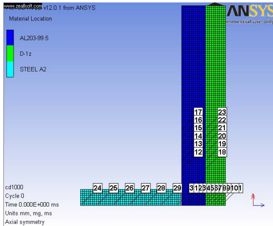
Figure 25. Autodyn® Simulation of an A2 Steel Cylinder Bullet Impacting at 1000m/s onto a Ceramic-D1 Composite Plate. (Left) Problem setup. (Right) Overall Pressure-Time profile.
