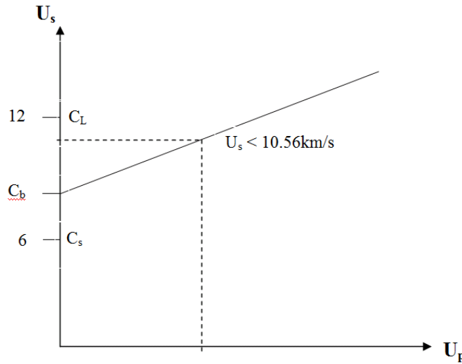
Figure 29. Possible Us-Up Relationship in the 22/33-Direction for D1 Material. (Not to Scale)
