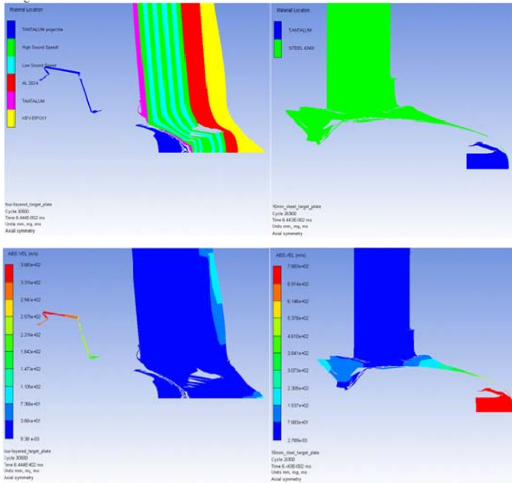
Figure 3. A Composite Plate Construction Was Shown By Poh To Defeat A Projectile Where A High Strength AISI 4340 Steel Had Failed.
