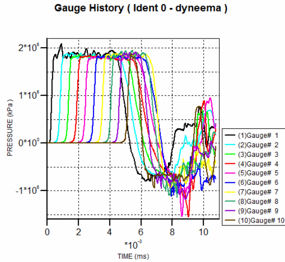
Figure 15. Gauge History of D1 Material Subjected to a Flyer Impact of the Same Material at 1km/s
