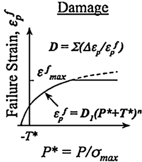
Figure 6. Graphical Interpretation of the Damage Constant, D (From [7])
