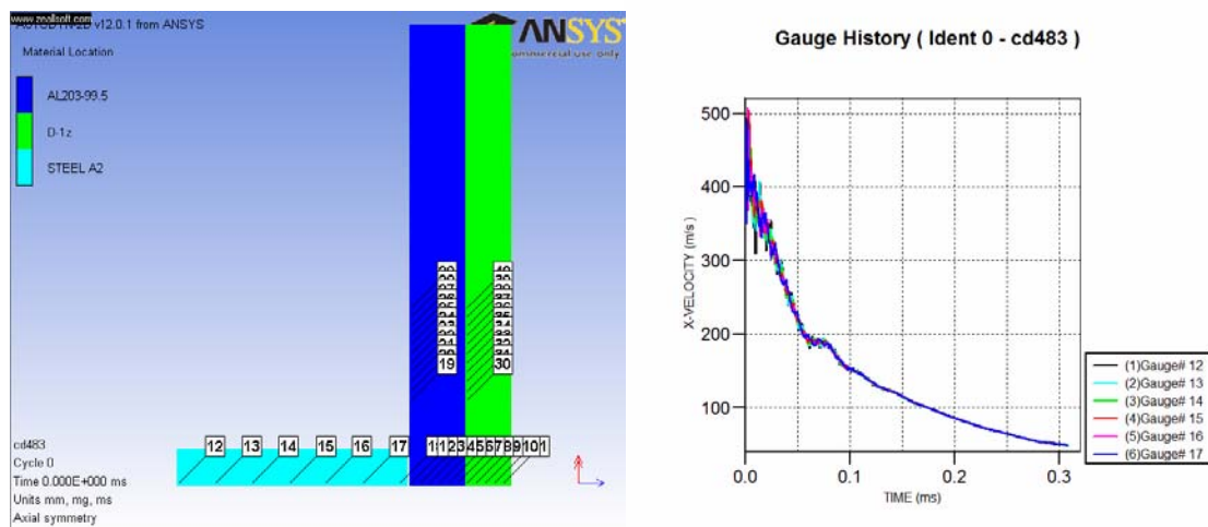
Figure 52. (Left) Problem Setup of 1” A2 Steel Cylinder Rod Impacting at 483 m/s onto a Composite Plate Comprising of Ceramic, and D1 (C-D1). (Right) Velocity Profile showing that the Projectile is stopped after about 0.32 ms.
