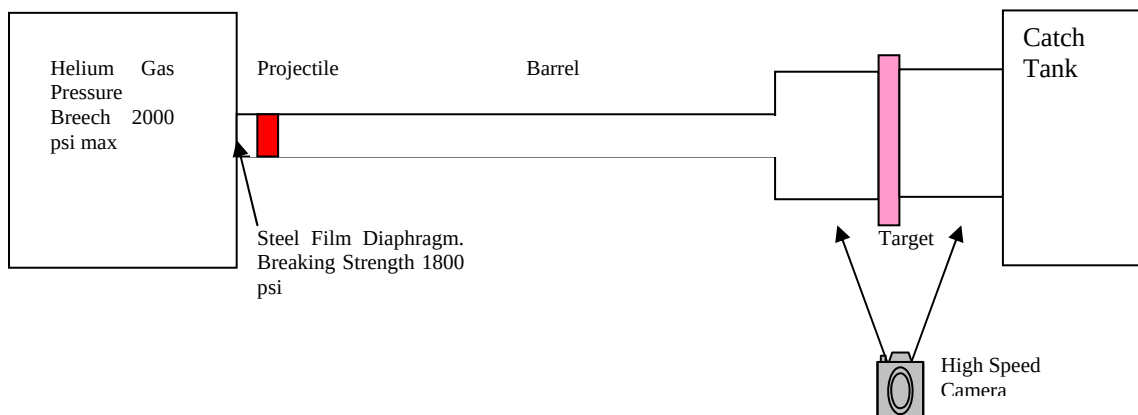
Figure 32. Schematic of the Gas Gun Facility
