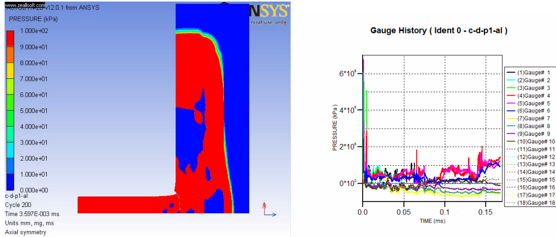
Figure 56. Shock Wave Propagation in the 11 and 22 directions. Overall Shock Pressure is Shown on the Right.
