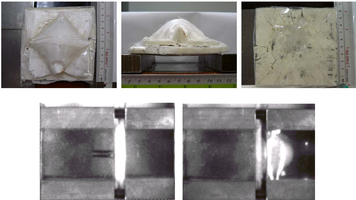
Figure 42. Sample of C-D Showing Complete Fracture of the Ceramic First Layer, and no Penetration of the Projectile.
