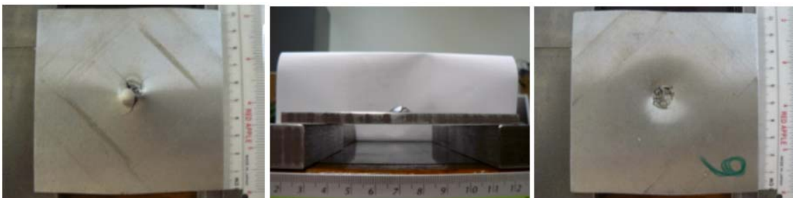
Figure 40. Target Samples and the Associated Damage of the AISI 4140 Steel Plate Impacted with 3/4" A2 Projectile at 500m/s. No Penetration was Observed.
