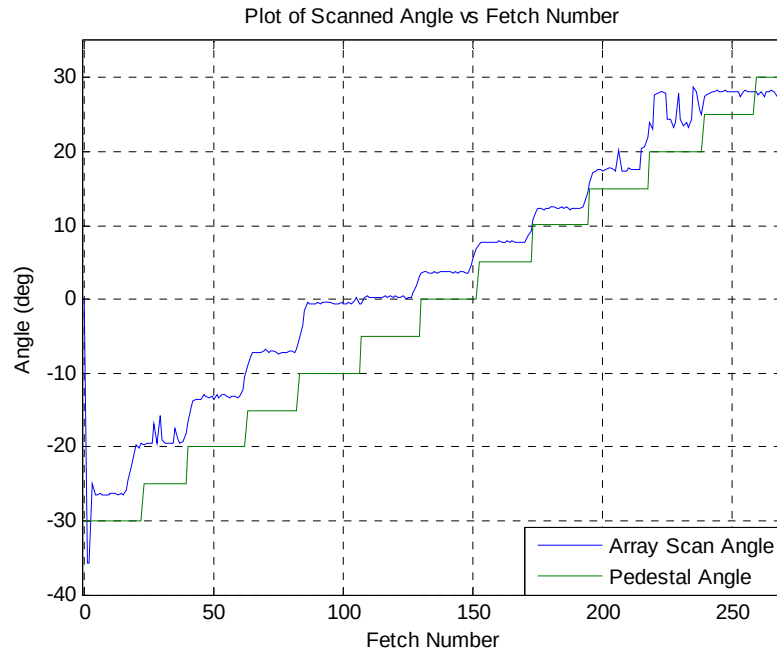
Figure 119. Plot of test 1 of angle against fetch number for AOA of -30^{\circ} to 30^{\circ} using RSNS for acquisition and DBF for tracking
