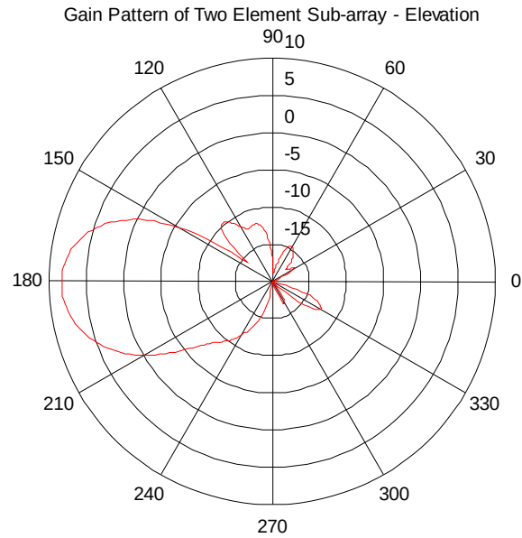
Figure 68. Measured elevation gain pattern
