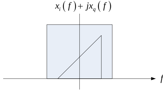
Figure 23. Final output with amplitude doubled
