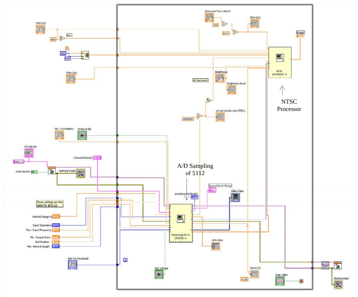
Figure 32. NTSC Decoding module
