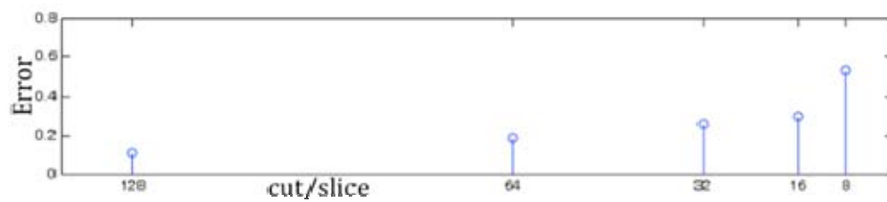
Figure 46. Cut and Slice results for FSK/PSK, signal only, including a stem plot of the error when compared to the original (top left).
