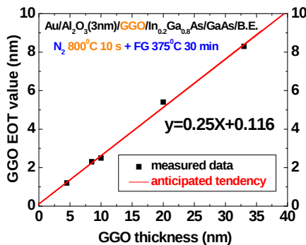
Scalability relationships between GGO thickness and EOT value
