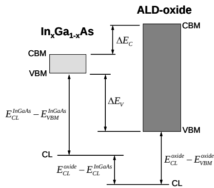
Schematic illustration of the energy band lineup at ALD-oxide/ \text{InGaAs} interface.
