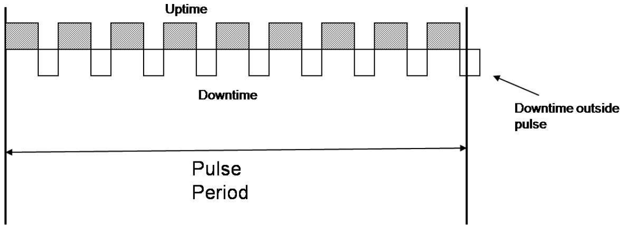
Figure 3. Pulse with many failure-restore cycles.
