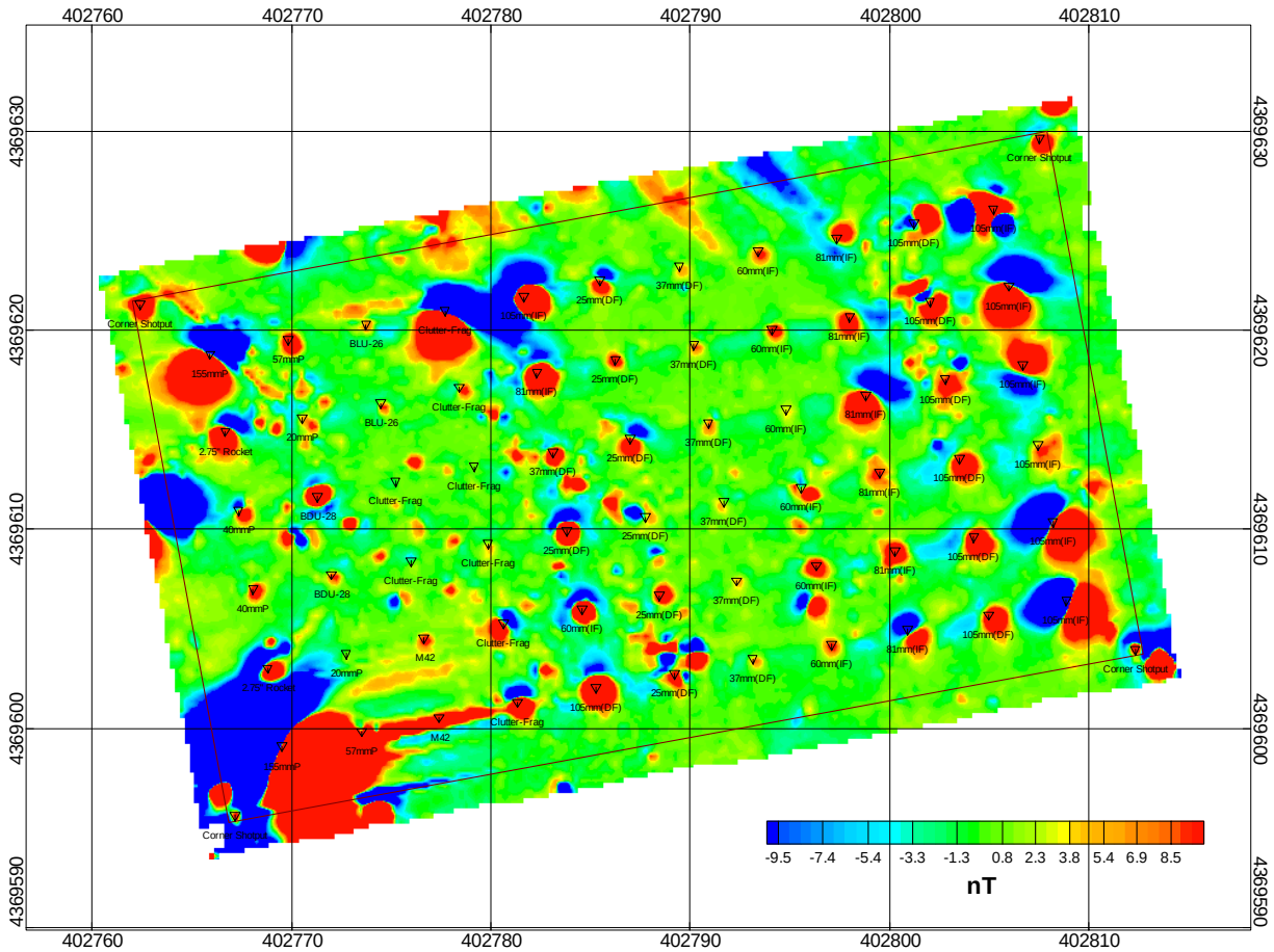
Figure 5-15 – Magnetometer anomaly map for the APG Calibration Area.
