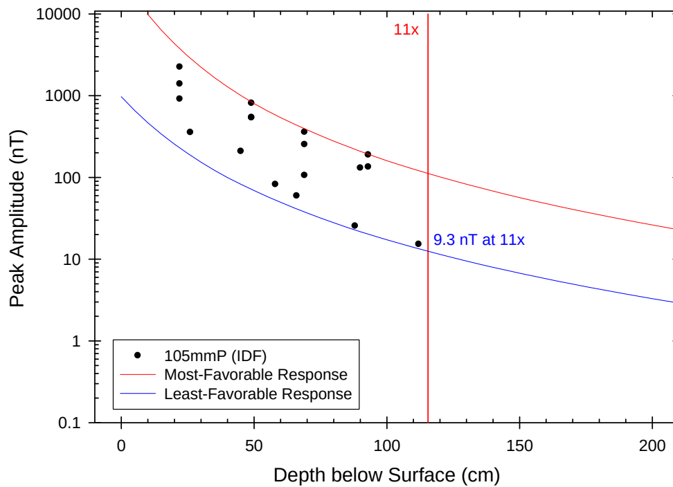
Figure 5-19 – Magnetometer response curve for the ATC standard 105mm Projectile
