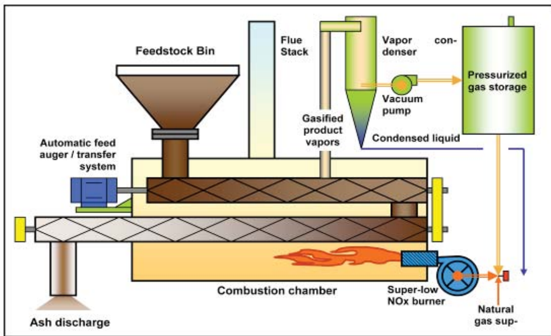
Figure 1.1-6 ACTI Gasification System Diagram
