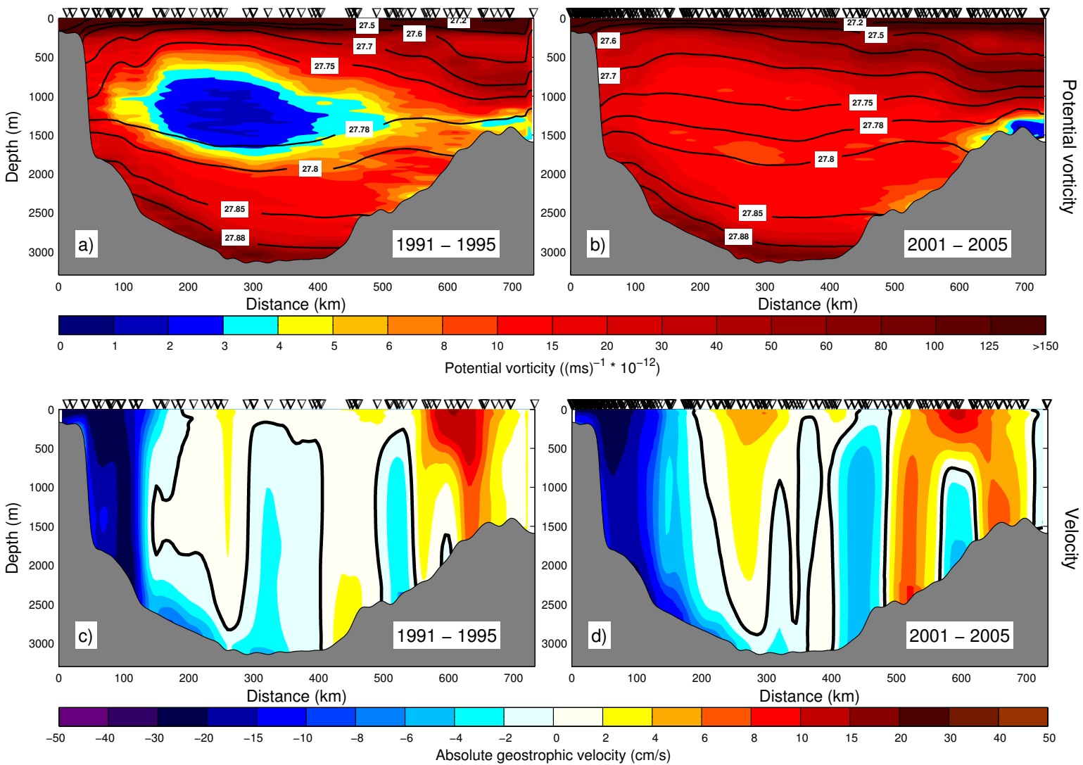
Figure 4-13: As in Figure 4-12, but for a, b ) potential vorticity ((\text{ms})^{-1} \cdot 10^{-12}) and c, d ) absolute geostrophic velocity (cm/s).
