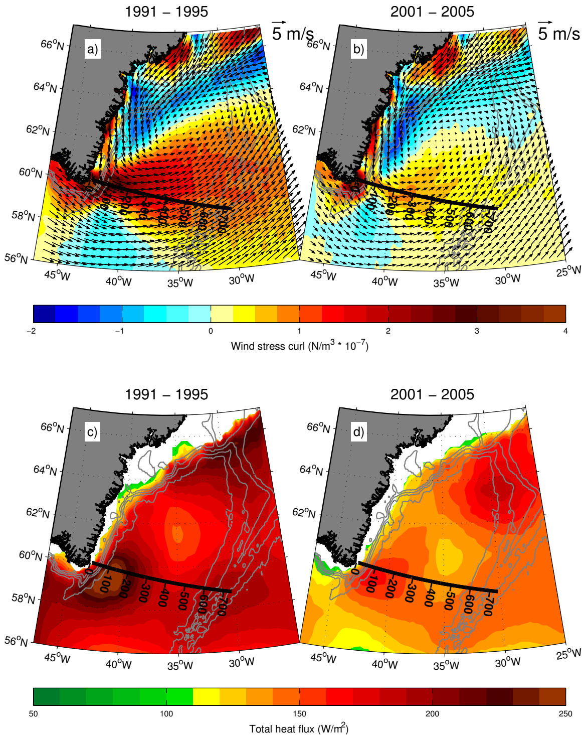
Figure 4-14: Maps of NARR winter a, b ) wind stress curl ( N/m^3 \times 10^{-7} ) and wind vectors ( m/s ) and c, d ) total turbulent heat flux ( W/m^2 ) averaged over the periods a, c ) 1991-1995 and b, d ) 2001-2005. The black line and numbers indicate the AR7E line and distance (in km ), depth is contoured with 500 m increments starting at 500 m .
