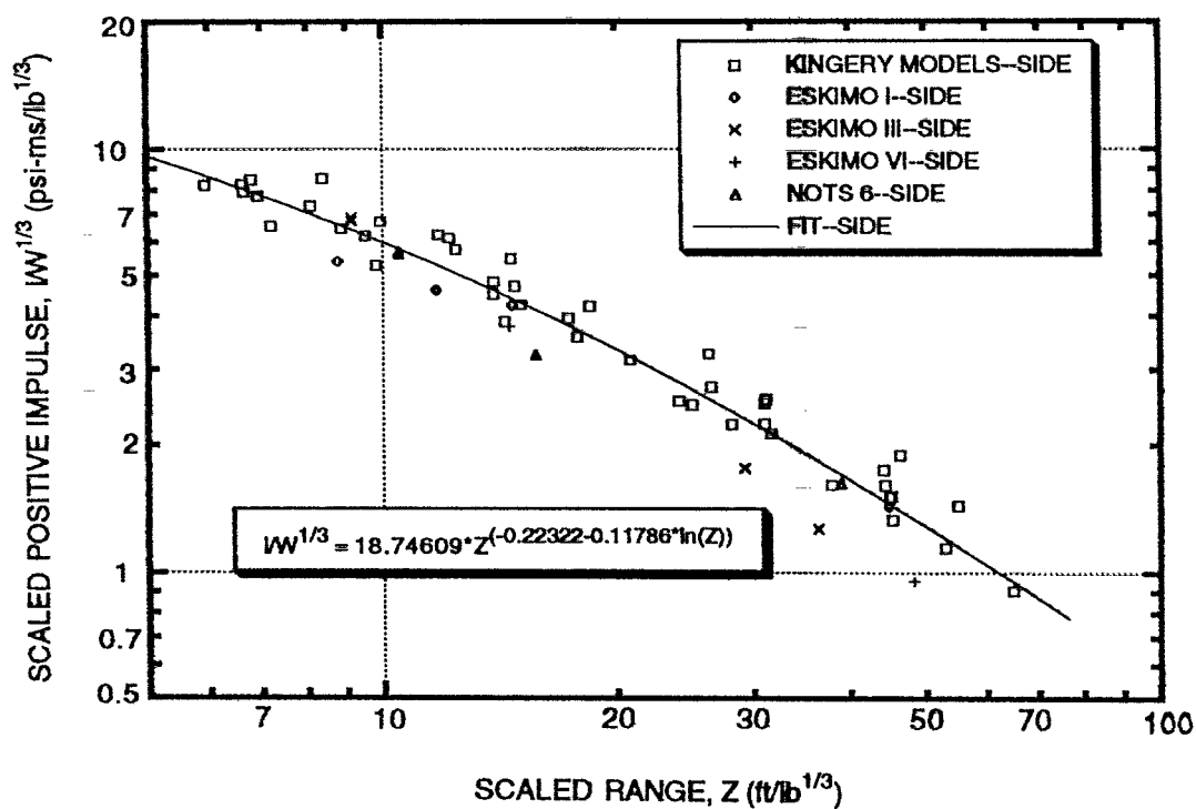
FIGURE 12. SCALED POSITIVE IMPULSE--SIDE
