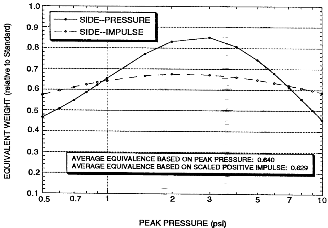
FIGURE 15. IGLOO EQUIVALENCE--SIDE
