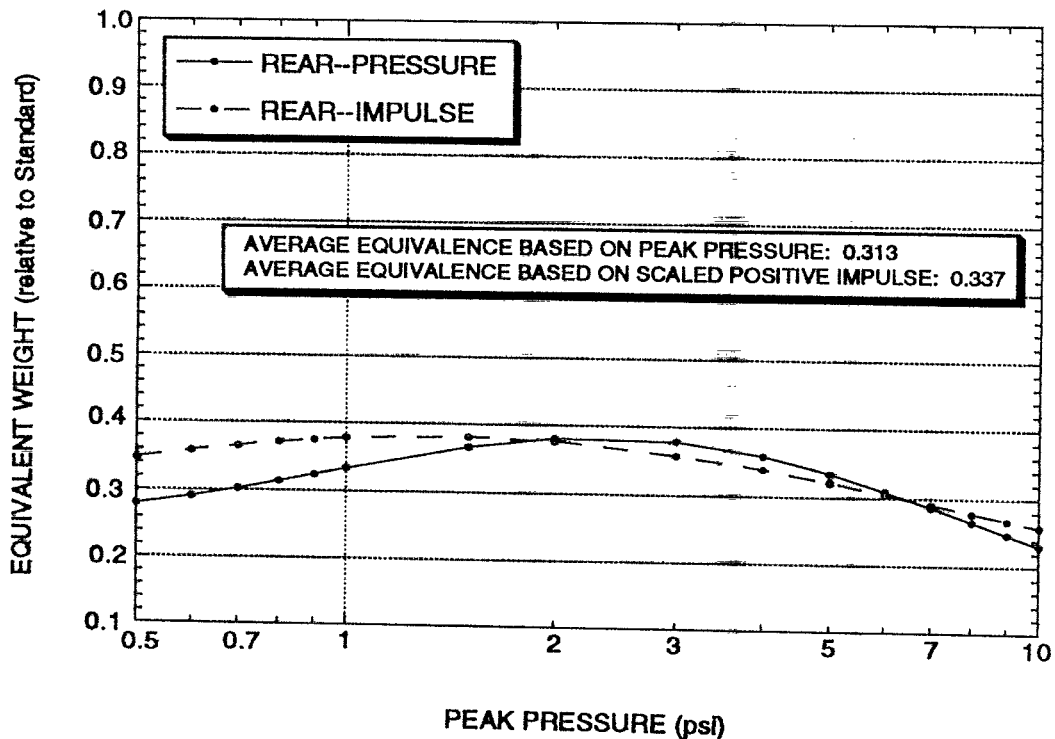
FIGURE 16. IGLOO IMPULSE--REAR
