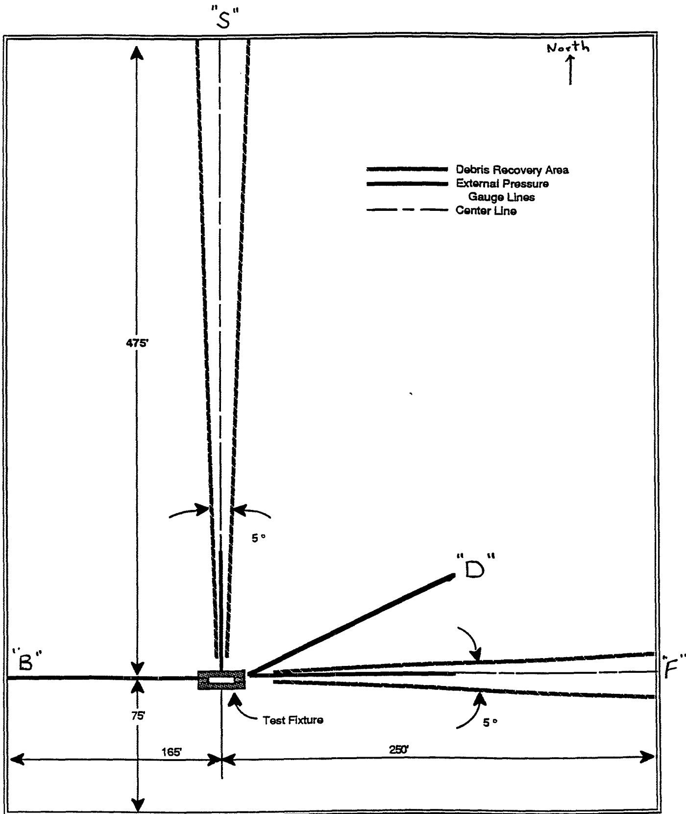
Figure 1. Overall site dimensions.
