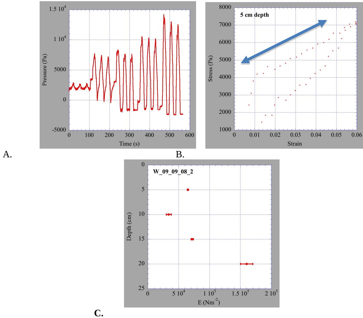
Figure 4. A. Pressure record from the E-probe from core W-09-09-08-2. B. The stress-strain diagram for the sediment at 5cm. The compressive slope (indicated by the blue line) is used to calculate E. C. The values of E as a function of depth for the W-09-09-08-2 core.
