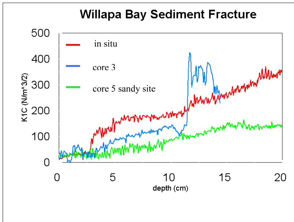
Figure 5. Measured K_{1C} (tensile fracture strength) with depth in 2 cores from Willapa Bay and an in situ profile from the site indicated in Fig. 1.
