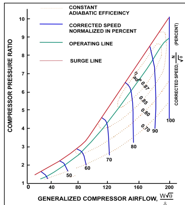
Figure 13. Typical Compressor Operating Map
