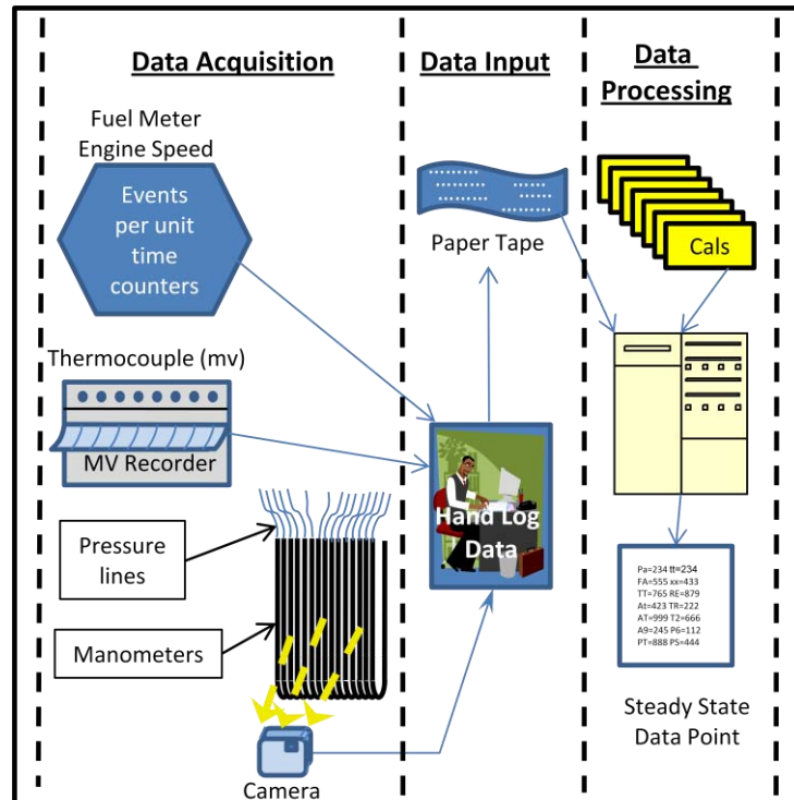
Figure 1. Data Acquisition and Processing Circa 1960
