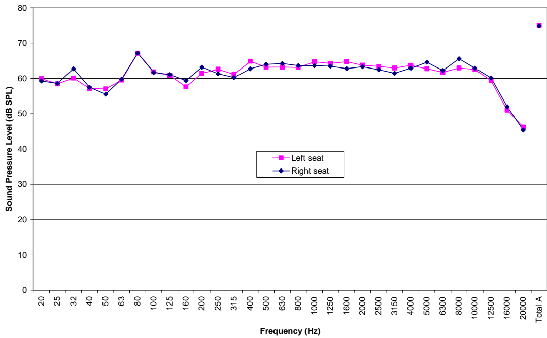
Figure 2: Background noise spectra (pink noise, total 75 dBA) at the two subject positions.
