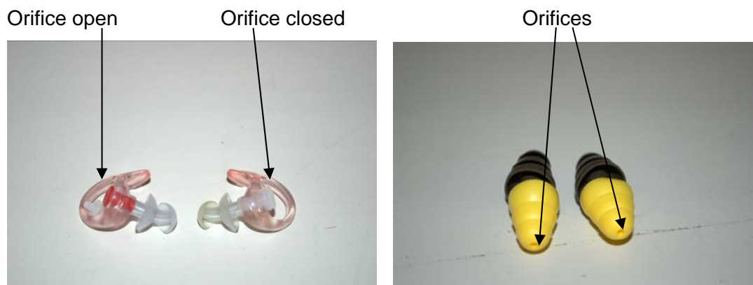
Figure 3: Left – Surefire EP3 Sonic Defender ™ earplugs; Right – E-A-R ® Combat Arms earplug.
