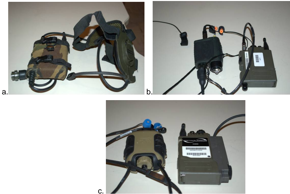
Figure 2: Personal role radio (PRR) with a) Standard headset (SH), b) Nacre QuietPro ® (QP), c) Silynx QuietOps ™ (QO).
