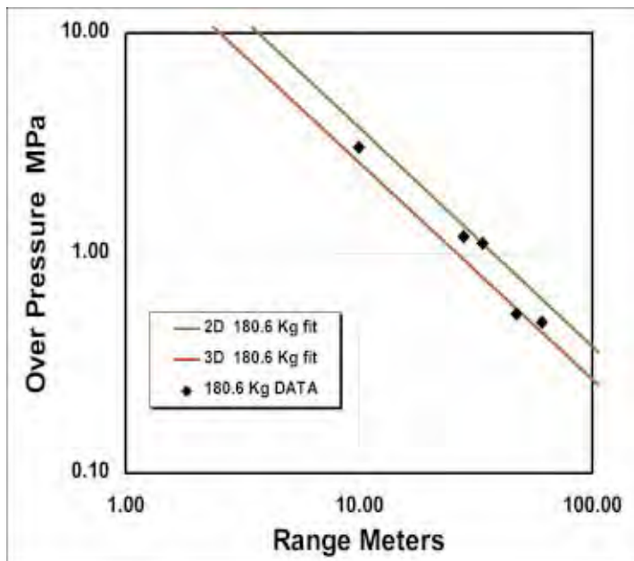
Figure 3. Comparison of pressure versus range from CTH 2-D and 3-D calculations
