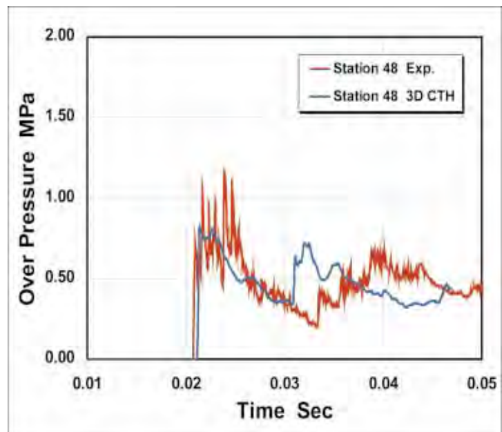
Figure 4. Comparison of pressure history from 3-D model with test results
