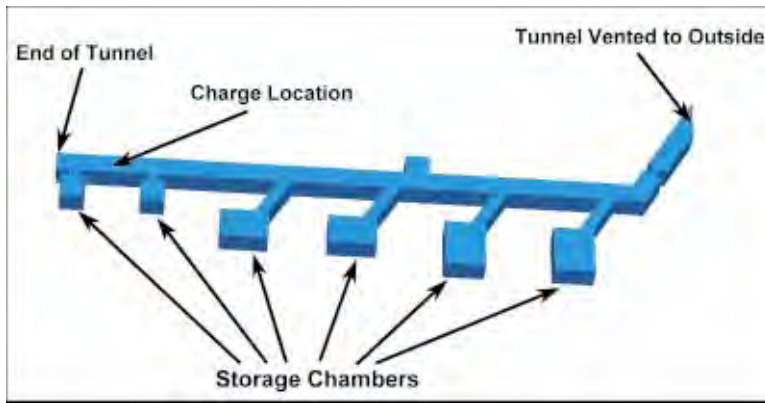
Figure 1. Full-scale tunnel layout
