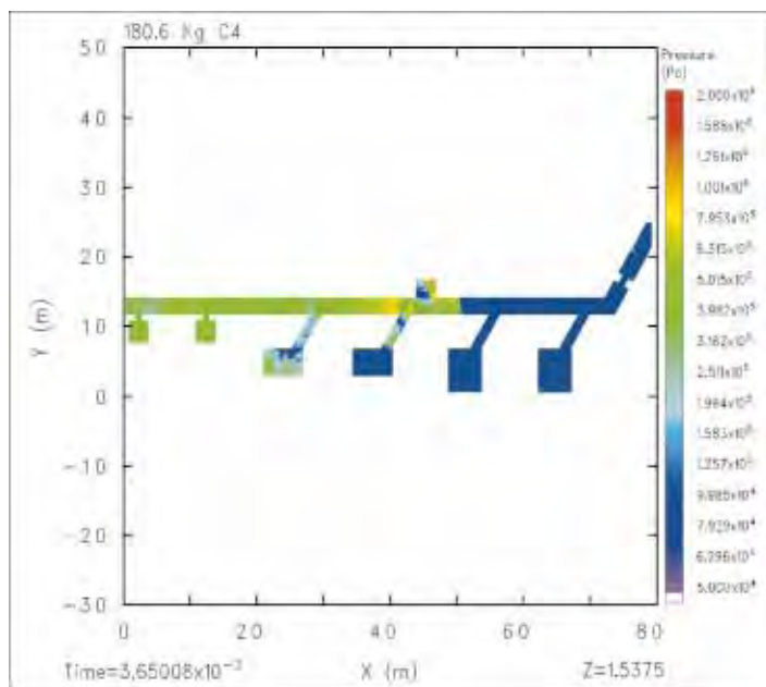
Figure 6. Blast wave propagation from 3-D calculations in tunnel after engulfment of storage tank
