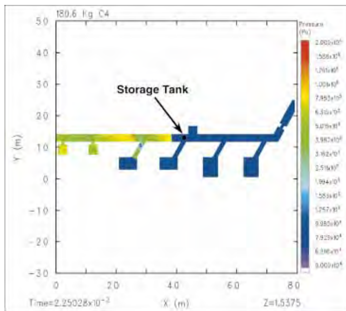
Figure 5. Blast wave propagation from 3-D calculations in tunnel before engulfment of storage tank
