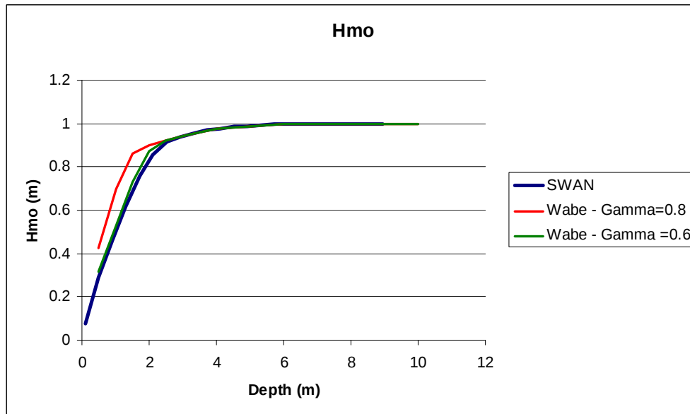
Figure 2: Comparison of significant wave height ( H_{mo} ) between SWAN (blue line) and the ray-trace code (Wabe) for two different values of the gamma parameter in the SWAN energy dissipation model for breaking waves. Note that the Wabe run with gamma = 0.6 is essentially identical to SWAN
