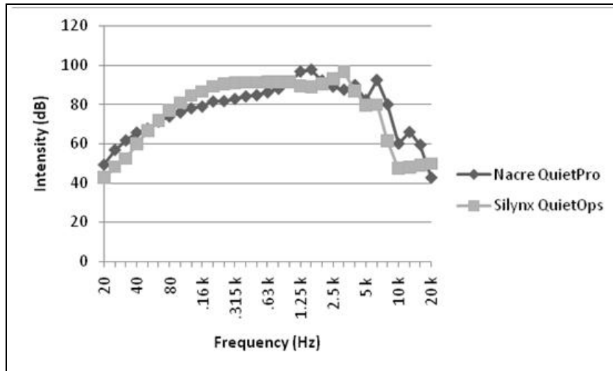
Figure 4. Frequency responses in 1/3 octave bands measured from the earphones of the two systems. The responses are equalized for the value at 1000 Hz. Frequency is shown on the x-axis and intensity is shown on the y-axis.
