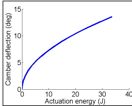
Figure 8 Camber deflection vs actuation energy for single cell adaptation
