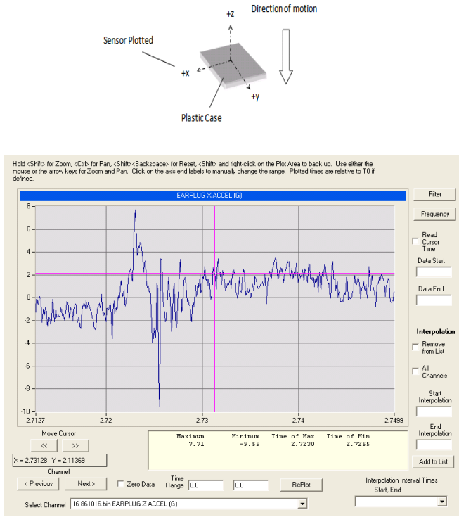
Figure 12. Plot of Model 7273GT X-axis Accelerometer
