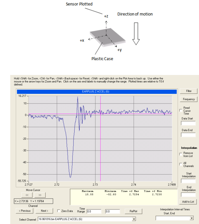
Figure 10. Plot of Model 7273GT Z-axis Accelerometer
