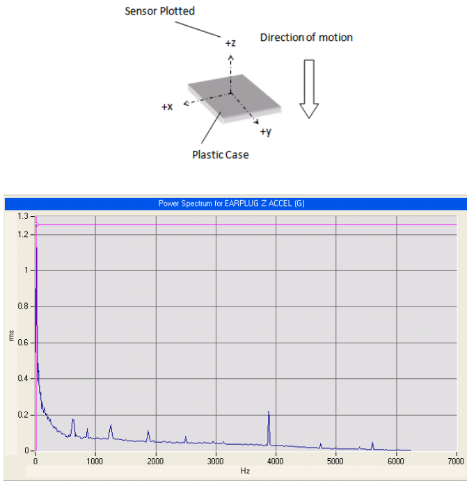
Figure 13. Power Spectrum Plots Used to Select Filter Frequencies
