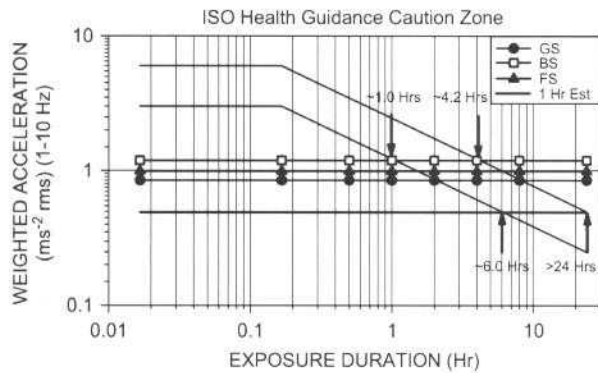
Fig. 7. ISO Health Guidance Caution Zones for locomotive seats based on Z-axis weighted seat pan accelerations for Signal 2. (Solid line is estimated weighted Z-axis seat pan acceleration for 1-hr field exposure. See Section 4.)
