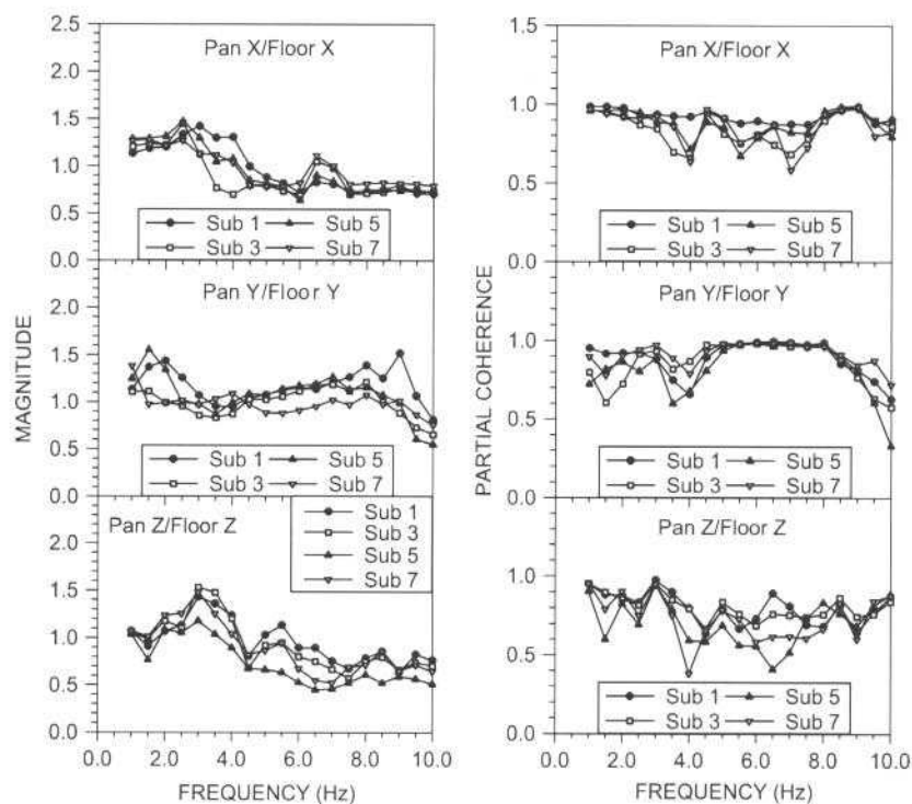
Fig. 5. Seat pan transmissibilities and partial coherences for Signal 2 exposure, GS seat (back-on). (Subject 1 = female, 53.6 kg; subject 3 = female, 94.0 kg, subject 5 = male, 75.6 kg, subject 7 = male, 96.5 kg.)
