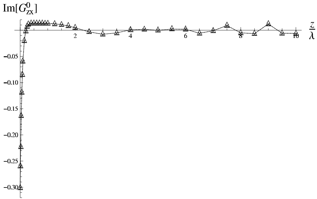
Fig. 22 — Behavior of the G_{zx}(\rho, z, \phi) Green's function vs. z/\lambda when observation point is outside the substrate. Here d = \lambda , \rho = 10\lambda , \phi = 0^\circ , \tan \delta = 0.0001 , and |\epsilon_{r1}| = 9.8 . The crosses ( \times ) refer to Eq. (32) and the triangles ( \triangle ) refer to direct MATHEMATICA computations. For Eq. (32), the breakpoint \xi_A = k_{max} = \Re(k_1) .
