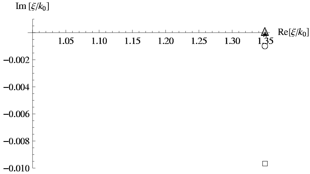
Fig. 13 — TM surface pole dispersion diagram vs. substrate loss tangents for a single layer PEC-backed substrate with thickness d/\lambda = 0.25 and |\epsilon| = 2.22 ; \tan \delta = 0.000(\triangle) , \tan \delta = 0.0001(\star) , \tan \delta = 0.001(\bigcirc) , and \tan \delta = 0.01(\square) .
