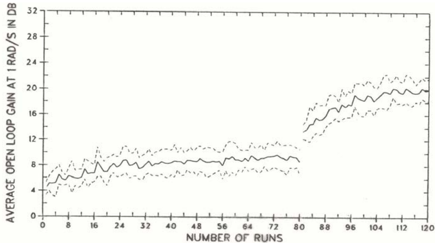
Figure 33. Open loop gain for the STATIC group
