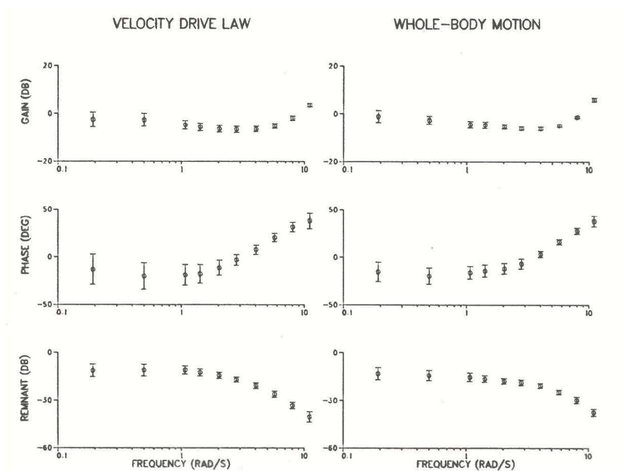
Figure 19. HODF for the VELOCITY group with remnant referred to the operator's input These data are averaged across the six group members and sixteen runs. The left figure reflects average control behavior late in the training environment (runs 65-80). The right figure shows data for late post-transition to the whole-body motion environment (runs 105-120). Mean values, plus and minus one standard deviation, are shown. The GAIN and PHASE curves characterize that portion of the operators' response linearly correlated with the input; the open-loop REMNANT, normalized by the error variance and referred to the operator's input, accounts for the remaining portion of the operator response. Zero db represents 1 lb control force per degree roll error for operator GAIN, and 1 \text{ (rad/s)}^{-1} for REMNANT.
