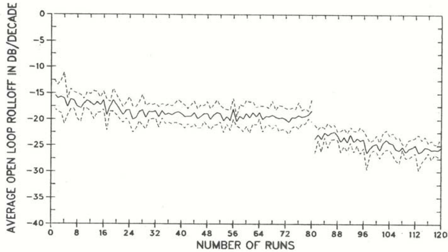
Figure 37. Open loop gain rolloff for the STATIC group
