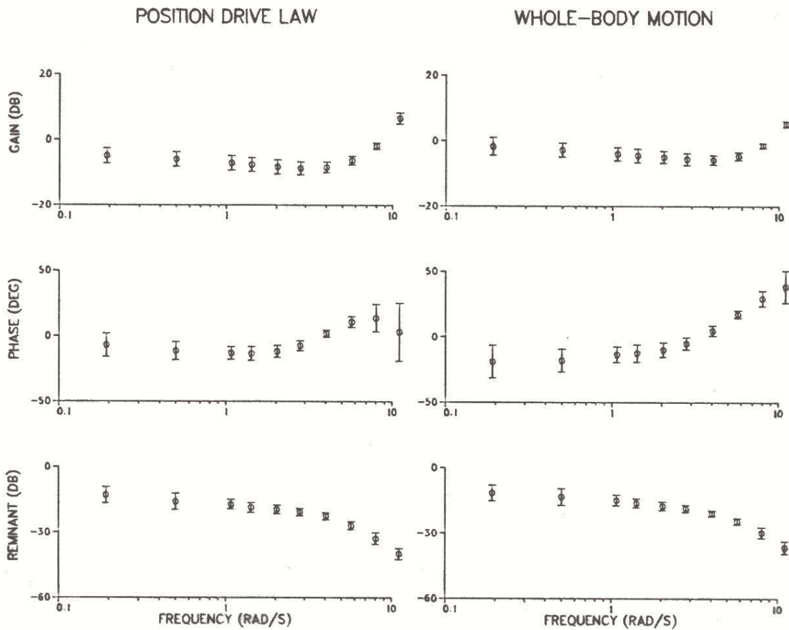
Figure 18. HODF for the POSITION group with remnant referred to the operator's input These data are averaged across the six group members and sixteen runs. The left figure reflects average control behavior late in the training environment (runs 65-80). The right figure shows data for late post-transition to the whole-body motion environment (runs 105-120). Mean values, plus and minus one standard deviation, are shown. The GAIN and PHASE curves characterize that portion of the operators' response linearly correlated with the input; the open-loop REMNANT, normalized by the error variance and referred to the operator's input, accounts for the remaining portion of the operator response. Zero db represents 1_lb control force per degree roll error for operator GAIN, and 1 (rad/s) -1 for REMNANT.
