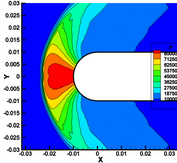
Figure 11(b) Pressure contours, B_0=5 , 11 species air
