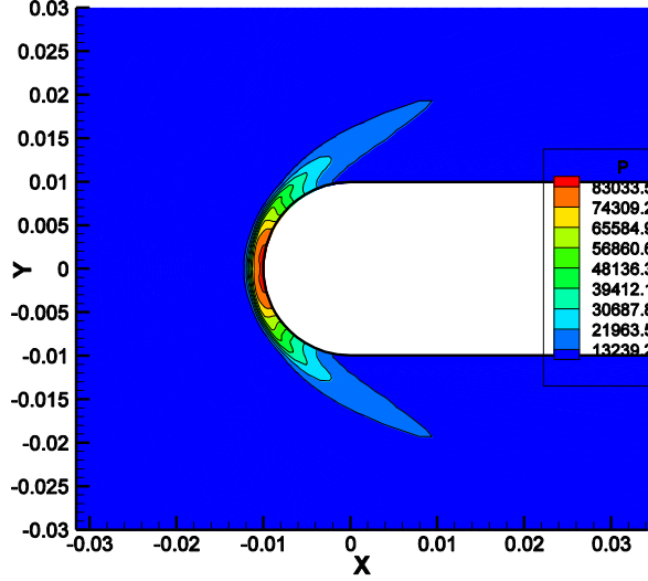
Figure 10 Pressure contours, B_0=0 , 7 species air
