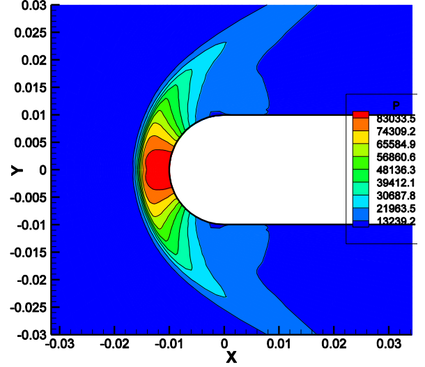
Figure 11(a) Pressure contours, B_0=5 , 7 species air
