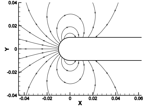
Figure 9 Dipole magnetic field lines
