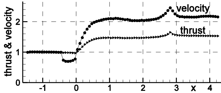
Figure 26 Accelerator Section Thrust and Velocity
