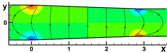
Figure 19 Imposed B_{0x} field
