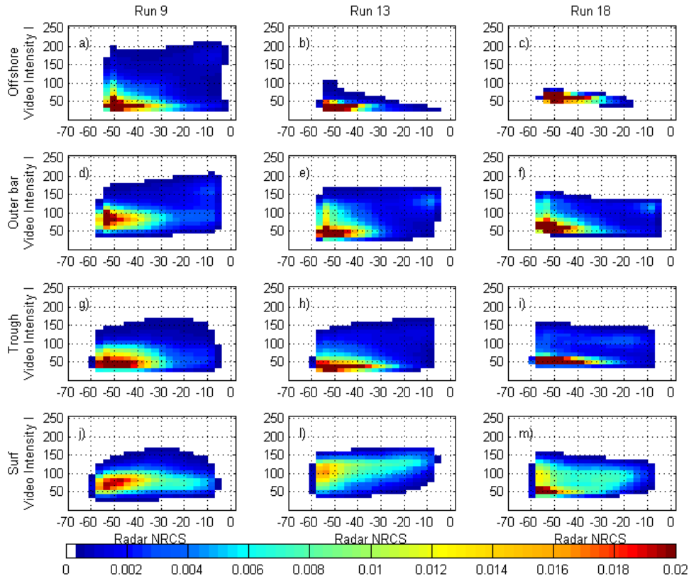
Figure 6: Joint Probability Density function for video (Camera 1) and Marine radar. Columns correspond to Runs 9, 13 and 18, respectively. Rows correspond to zones within the surf.
