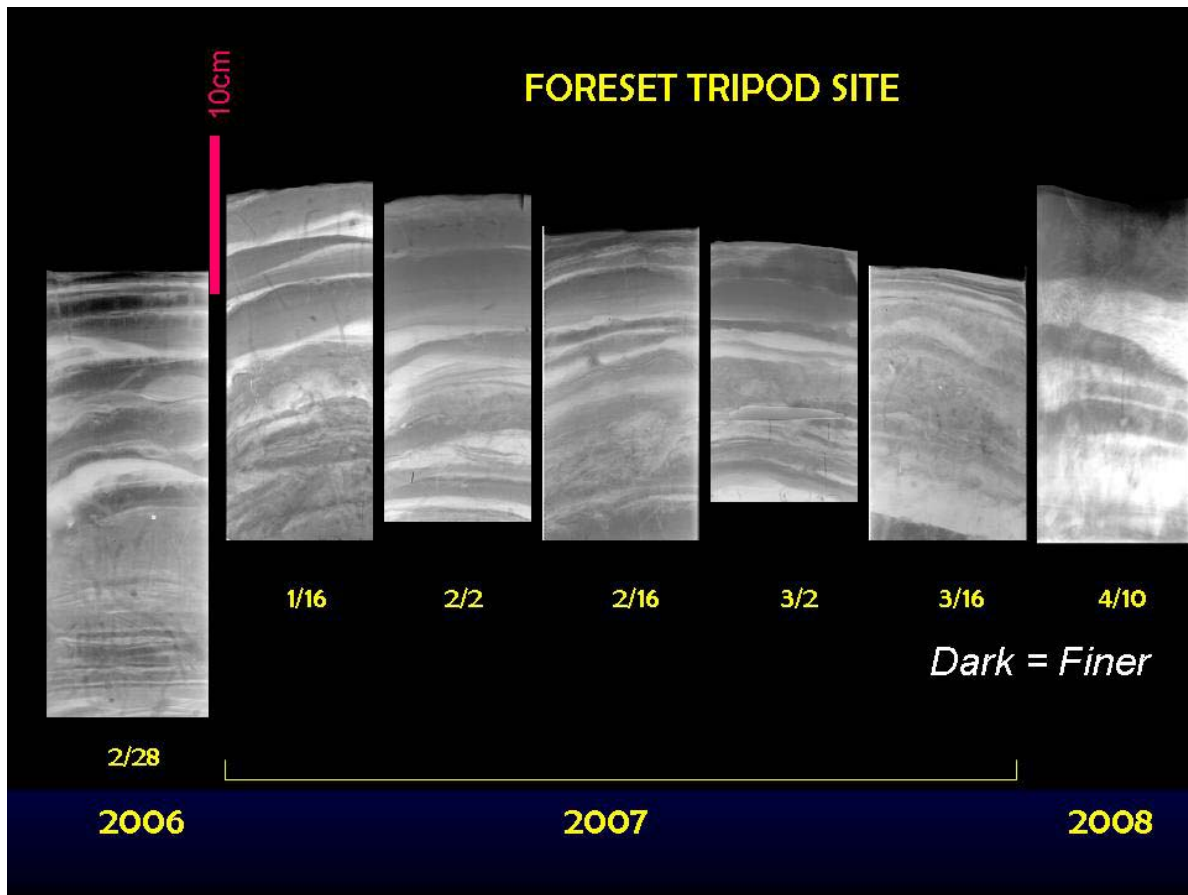
Figure 5. X-radiograph positives (dark=finer sediment) of upper seabed stratigraphic evolution at the foreset (T1) site taken from cores collected during two week turnarounds of the tripods. Only one date is shown in 2006 and 2008, while all the 2007 dates are shown. These data demonstrate the complex response of upper seabed stratigraphy to the multiple frontal storms experience yearly and are likely a combination of normal resuspension-deposition cycles (smaller events) and fluid-mud depositional events (larger events).
