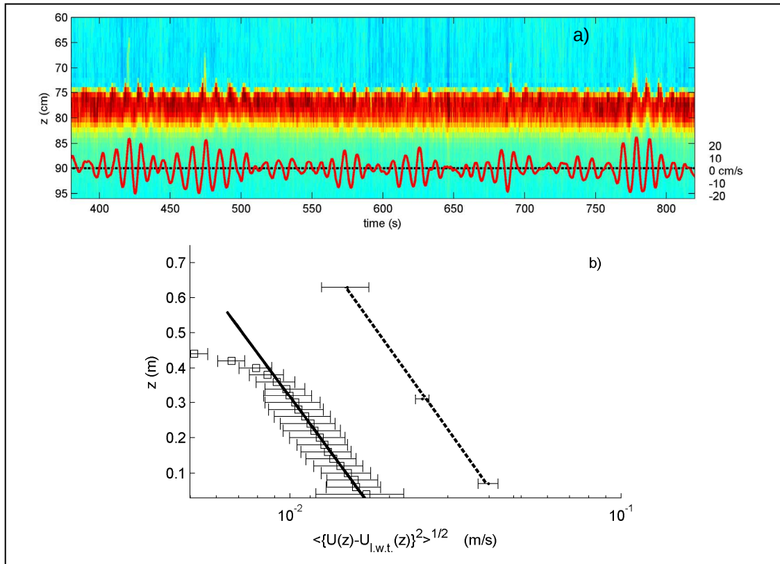
Figure 2. a) 400 seconds of 2 Hz sampled 2.5 MHz ABS data showing u_{0.1:3} \pm 2 cm amplitude oscillations on the lutocline. A time series of cross-shore velocity from an ADV located 75 cmab is also shown (red). This data burst was collected on day 35.56 as shown by the green line after event 3 in figure 2. b) Vertical profile of \langle U(z) - U_{l.w.t.}(z) \rangle from the 5 m site pulse Coherent ADCP (solid line and squares) for the 5 hourly data bursts proceeding and including that shown in panel a and the vertical array of ADVs at the 7 m site (dashed line and dots). Least squares fits to data from 0.05 m < z < 0.35 m are shown with a mean slope over all bursts of k_{int} = 1.8 \text{ m}^{-1} and intercept of u_{0,int} = 0.018 \text{ m/s} for the 5 site and 0.044 \text{ m/s} for the 7 m site .
