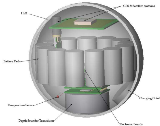
Figure 1. Cross-Sectional Schematic View of Riverine Drifter.
