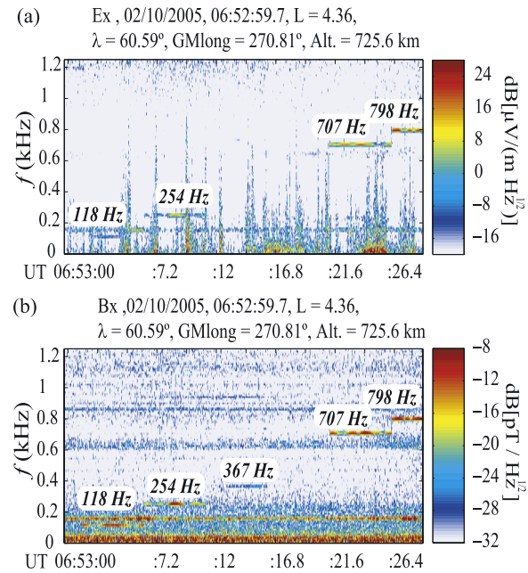
Figure 3. Detailed ICE and IMSC spectrograms from the DEMETER satellite pass during February 10, 2005. (a) An overview of the detected HAARP signal in one of the electric field components. The transmitted pattern at frequencies up to 798 Hz is observed. (b) An overview of the detected HAARP signal in one of the magnetic field components. The transmitted pattern at frequencies up to 798 Hz is observed.
