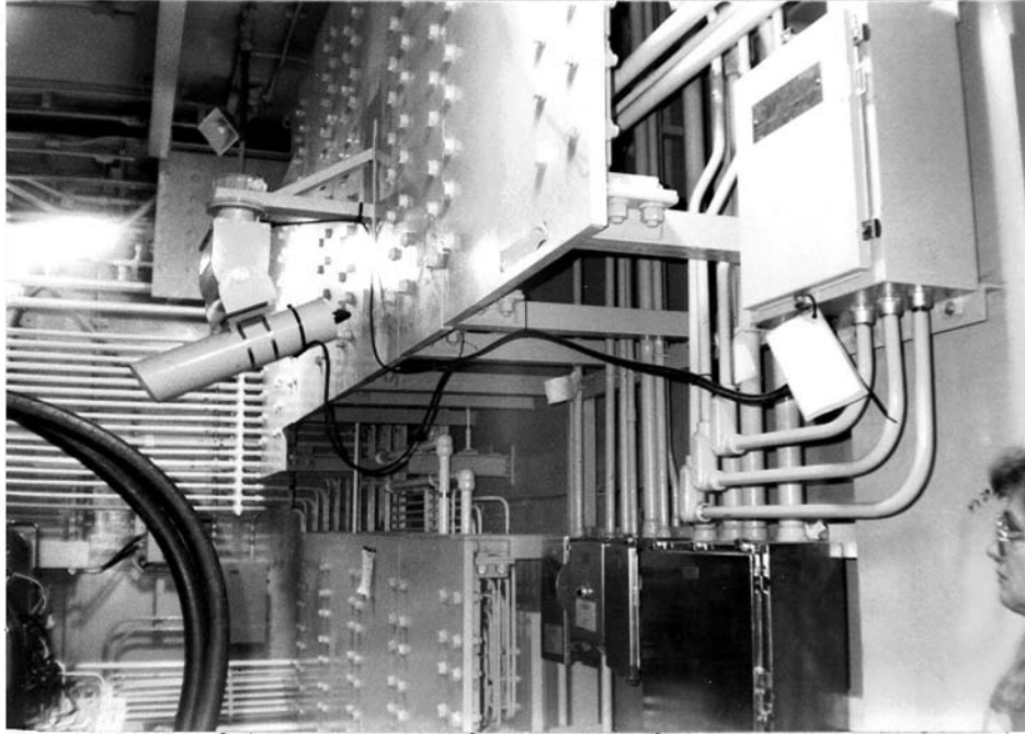
Fragmentation shield in ECR
