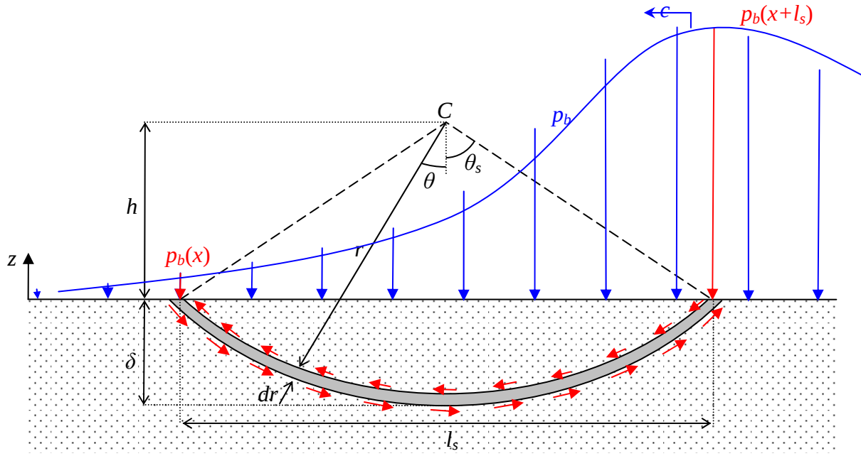
Figure 1: Geometry and force balance for a slip annulus.
