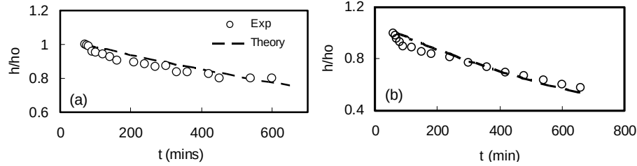
Fig. 5. The time decay of the dimensionless ripple height h/h_0 under weak oscillatory flow for two experiments (a, b) with different forcing (specified by frequency \omega and amplitude \varepsilon of oscillations). Symbols – measurements, dashed lines – predictions (1). The flow was applied on established ripples when h/h_0 = 1 .
